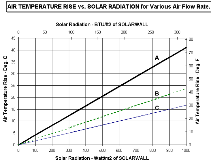
Graph illustrating temperature rise vs. solar radiation intensity. A low flow rate, C high flow rate. ( www.solarwall.com )
