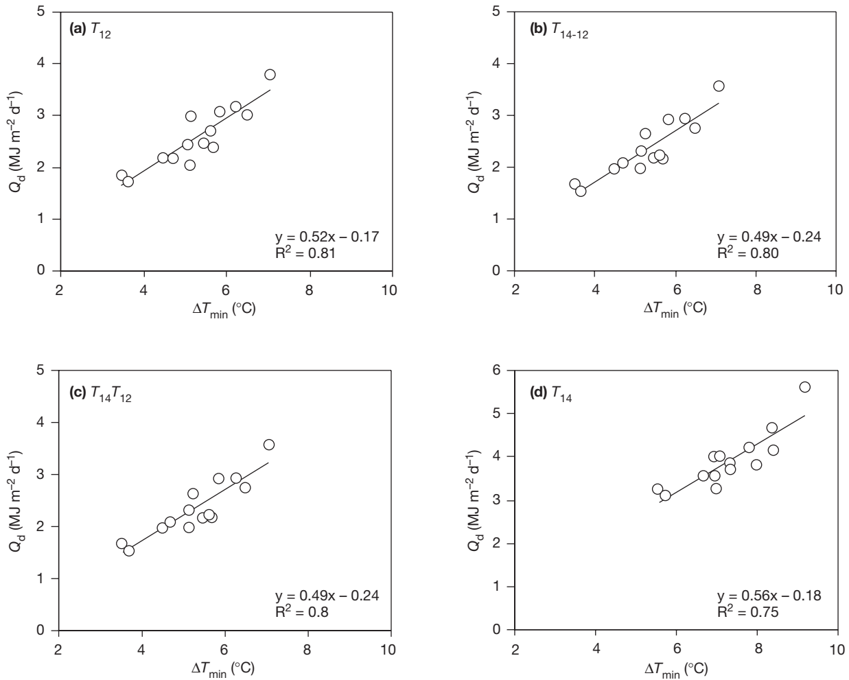
Figure 4. Daily heat consumption ( Q_d , MJ m -2 d -1 ) vs daily temperature difference ( \Delta T_{\min} ) between the heating set-point temperature and the minimum outside air temperature under treatments (a) T_{12} , (b) T_{14-12} , (c) T_{14}T_{12} and (d) T_{14} .
