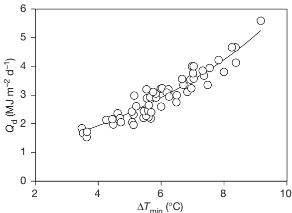
Figure 5. Daily heat consumption ( Q_d , MJ m -2 d -1 ) vs daily temperature difference ( \Delta T_{\min} ) between the heating set-point temperature and the minimum outside air temperature. Pooled data of heating treatments: T_{12} , T_{12-14} , T_{12}T_{14} and T_{14} .
