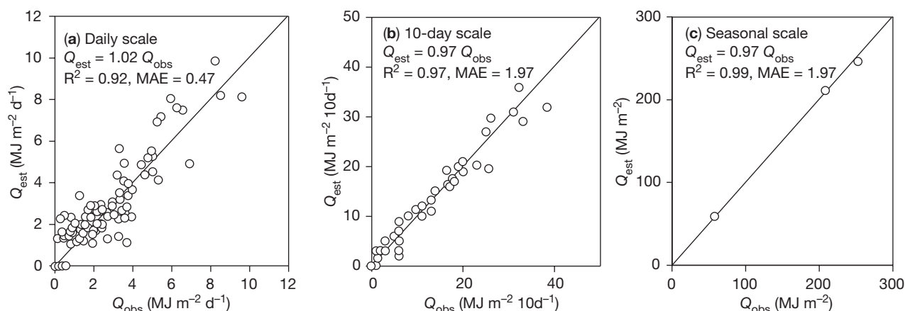
Figure 9. Estimated ( Q_{est} ) versus observed ( Q_{obs} ) values of heat consumption at (a) daily, (b) ten-day, and (c) seasonal scales. MAE: mean absolute error. Pooled data of the three validation treatments.
