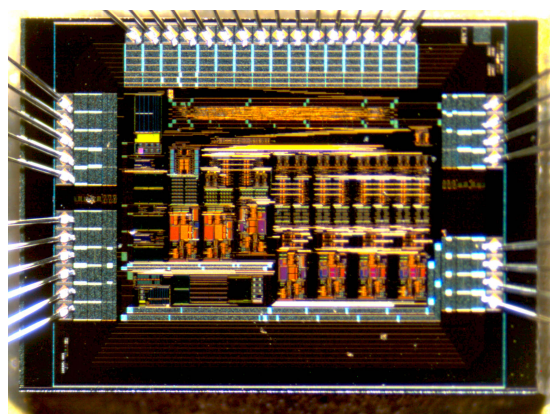
Figure 9. Chip microphotograph of the ADC with partial OTA sharing.
