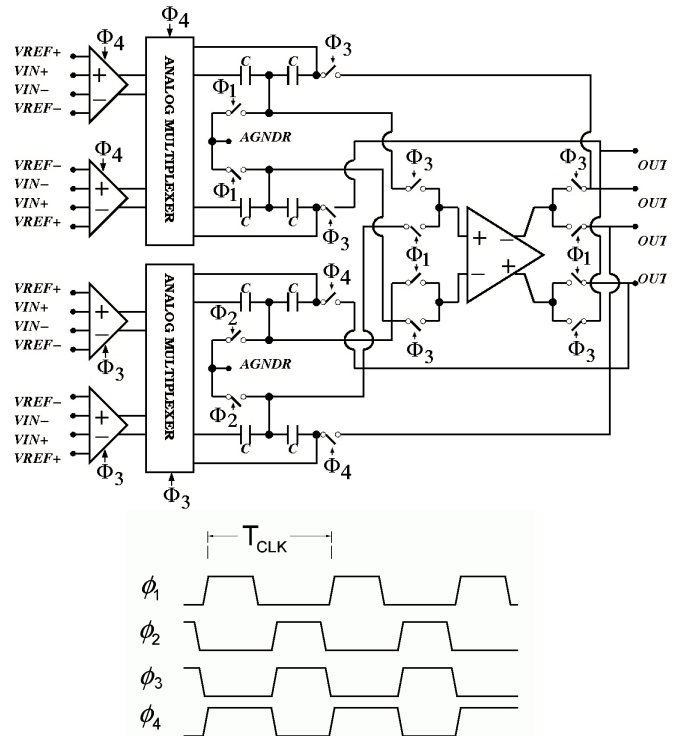
Figure 5. Structure of two stages with opamp sharing.
