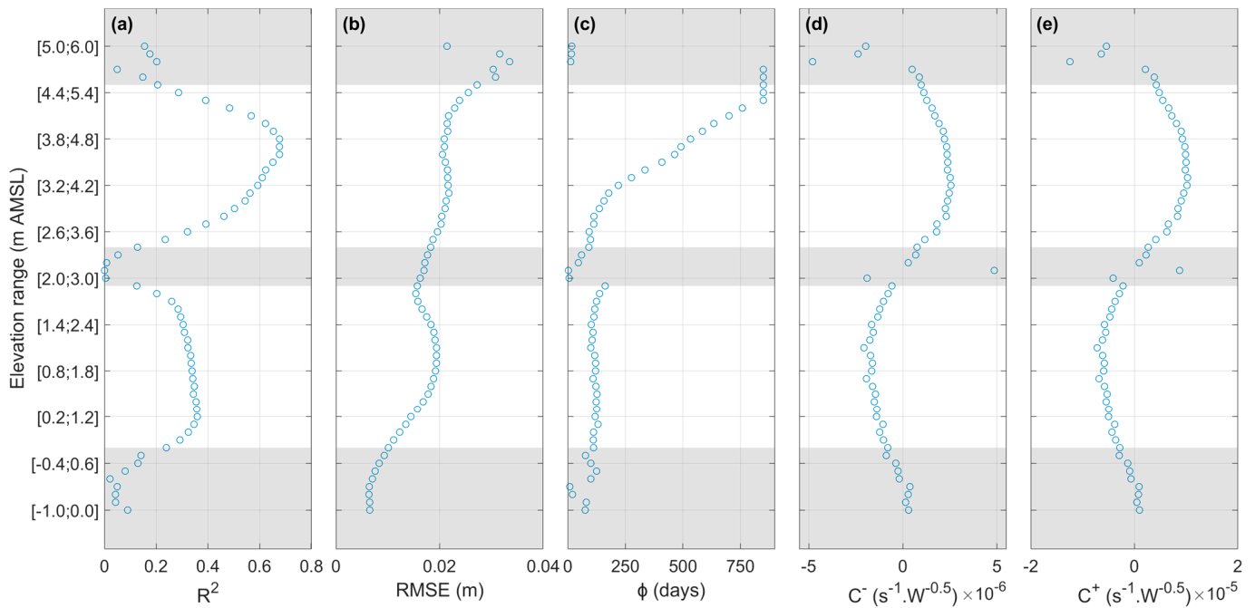
Figure 5. (a) R^2 and (b) RMSE between the observed and modeled beach slope and corresponding (c) \Phi memory, (d) C^- erosion rate coefficient and (e) C^+ accretion rate coefficient free parameters, found as a function of the elevation where the beach slope is computed. The shaded areas are where R^2 < 0.2 which we considered as elevations where beach slope does not show an equilibrium response.
