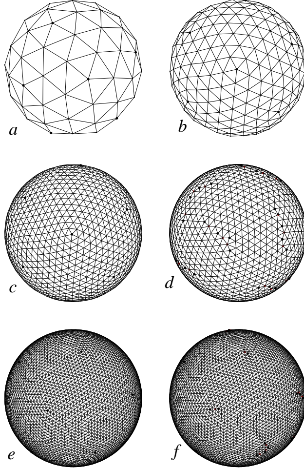
FIG. 1: Tetrahedral configurations. For a ) N = 78 ( E = 2662.04647 ), b ) N = 306 ( E = 43862.56978 ), the symmetric tetrahedral lattice configuration appears to be the global energy minimum, while for N = 1218 c ) ( E = 718284.03747 ), d ) ( E = 718281.63110 ) and N = 4886 e ) ( E = 11651484.51295 ), f ) ( E = 11651440.24177 ) addition of defects to the lattice produces a configuration of lower energy. For N = 1218 and 4886 we give the lowest energy configuration we have found, though we cannot certain this is a global energy minima. Fivefold coordinated charges (points) (pentamers) are indicated by large black dots, and sevenfold coordinated charges (septamers) are indicated by small red dots. The rest of the charges are sixfold coordinated (hexamers). Colors in online version only.
