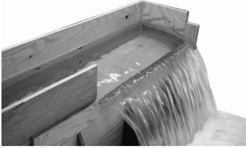
Figure 5 Physical model of side weir
