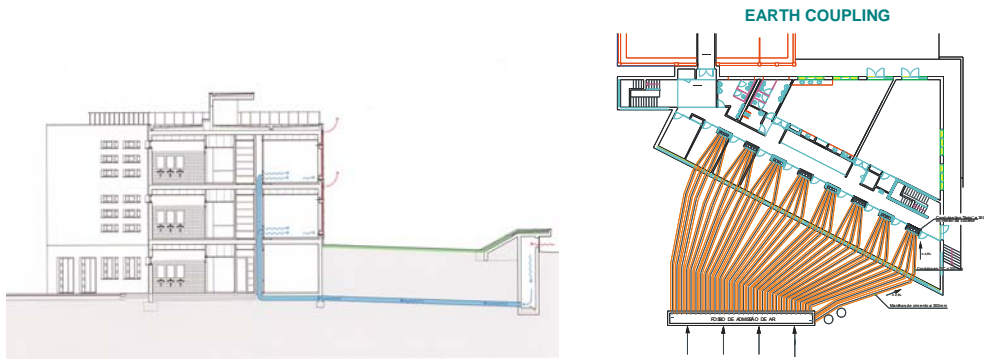
Earth coupling system and cooled air supply.
