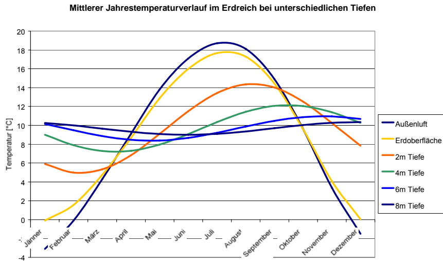
Annual temperature of outdoor air, surface of the earth and earth at different depths for the soil types “pebble stones –dry“, location Graz. The graph is based on the mean monthly values.
