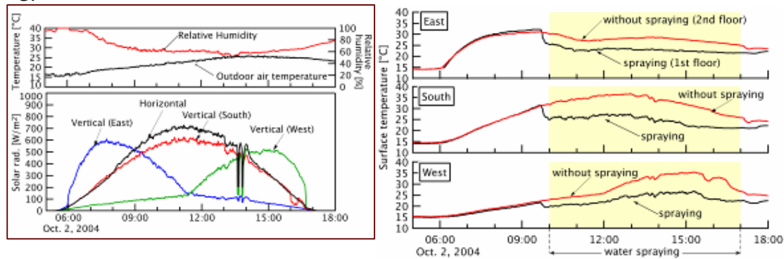
Outdoor climate of a day used for discussion
