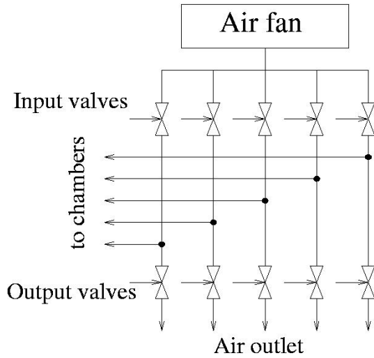
Figure 4: Fan/valve system.
