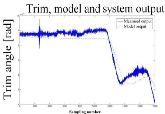
Figure 9: Trim simulated and measured (Andersen, 2007).
