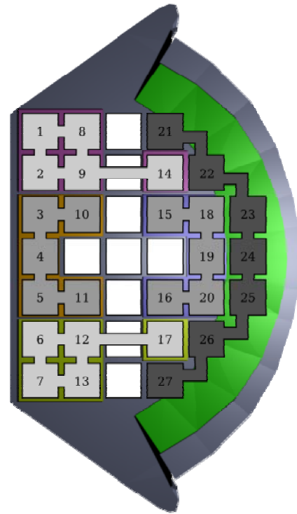
Figure 3: The air chambers in the Wave Dragon.
