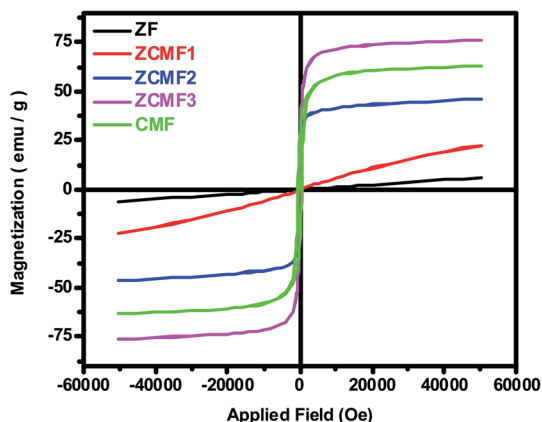
Fig. 5 Magnetic hysteresis loops of the Zn_{1-x}Co_{0.5x}Mg_{0.5x}Fe_2O_4 ferrites.
