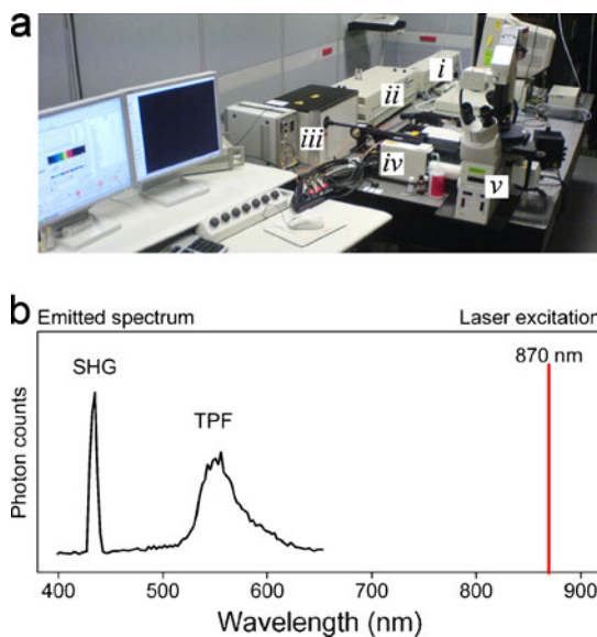
Fig. 2 Experimental setup for second harmonic generation (SHG) imaging. a Photograph of the laboratory room showing (i) pump laser, (ii) femtosecond pulsed IR laser (fs-laser), (iii) beam alignment, (iv) microscope confocal scanning module, and (v) inverted microscope. b Emission
