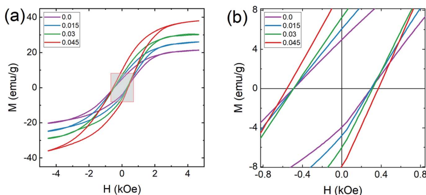
Fig. 8 Magnetization curves of Co 0.4 Cu 0.1 Zn 0.5 Dy x Fe 2-x O 4 . (a) Magnetization ( M ) as a function of applied magnetic field ( H ) and (b) expanded view of the M – H plots at low applied magnetic field strengths.
