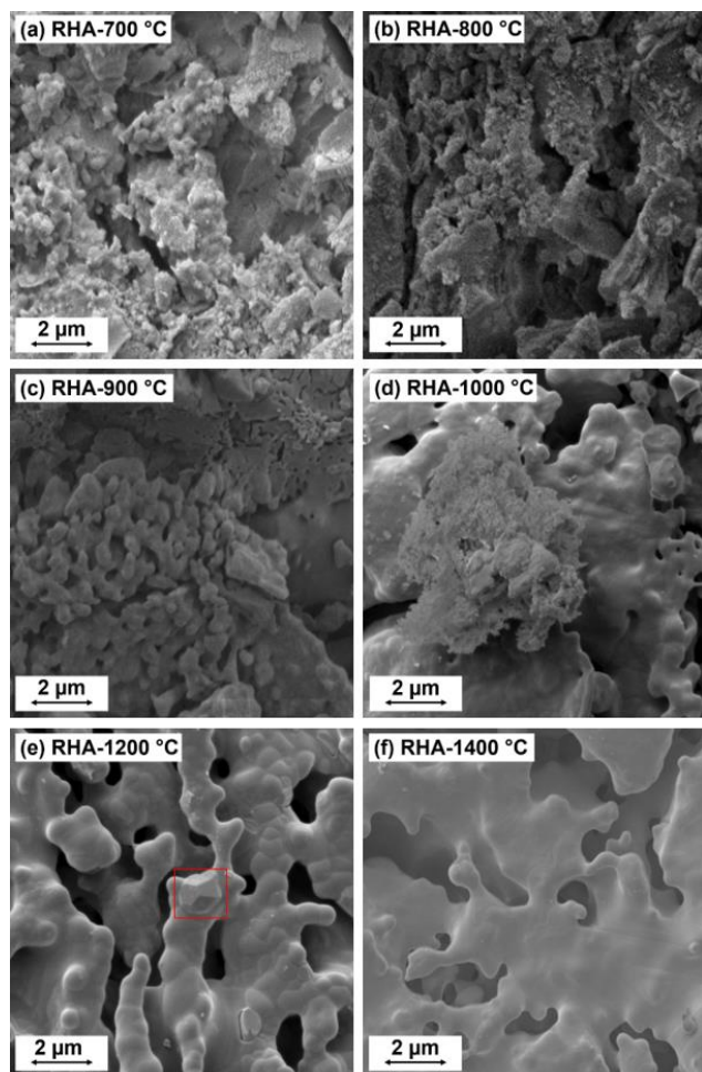
Fig. 4. FESEM micrographs for RHA produced from the sintering at (a) 700 °C, (b) 800 °C, (c) 900 °C, (d) 1000 °C, (e) 1200 °C and (f) 1400 °C, respectively.
