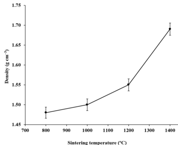
Fig. 3. Bulk densities for RHA produced from the sintering at 800, 1000, 1200 and 1400 °C, respectively.
