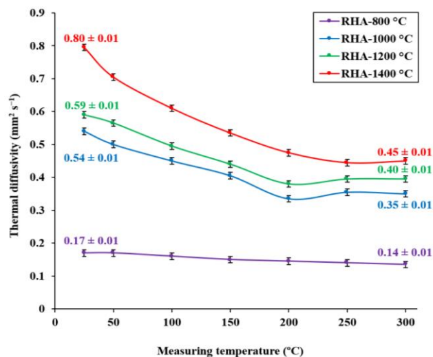
Fig. 5. Thermal diffusivity behaviours for RHA produced from the sintering at 800, 1000, 1200 and 1400 °C, respectively.
