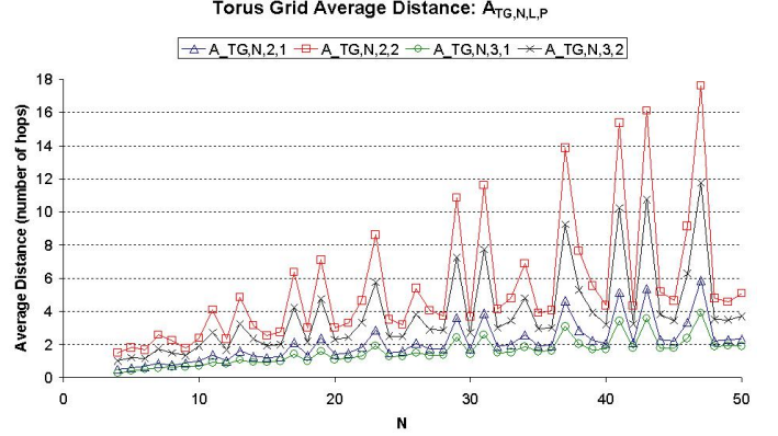
Fig. 9. Torus Grid, Average Distance for L=2 and P=1 ; L=2 and P=2 ; L=3 and P=1 ; and L=3 and P=2 respectively
