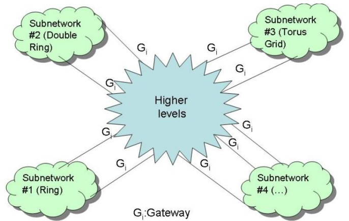
Fig. 1. Network Scheme
