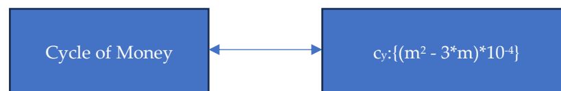
Figure 1. Cycle of money for c_y: \{(m^2 - 3 \cdot m) \cdot 10^{-4}\}
