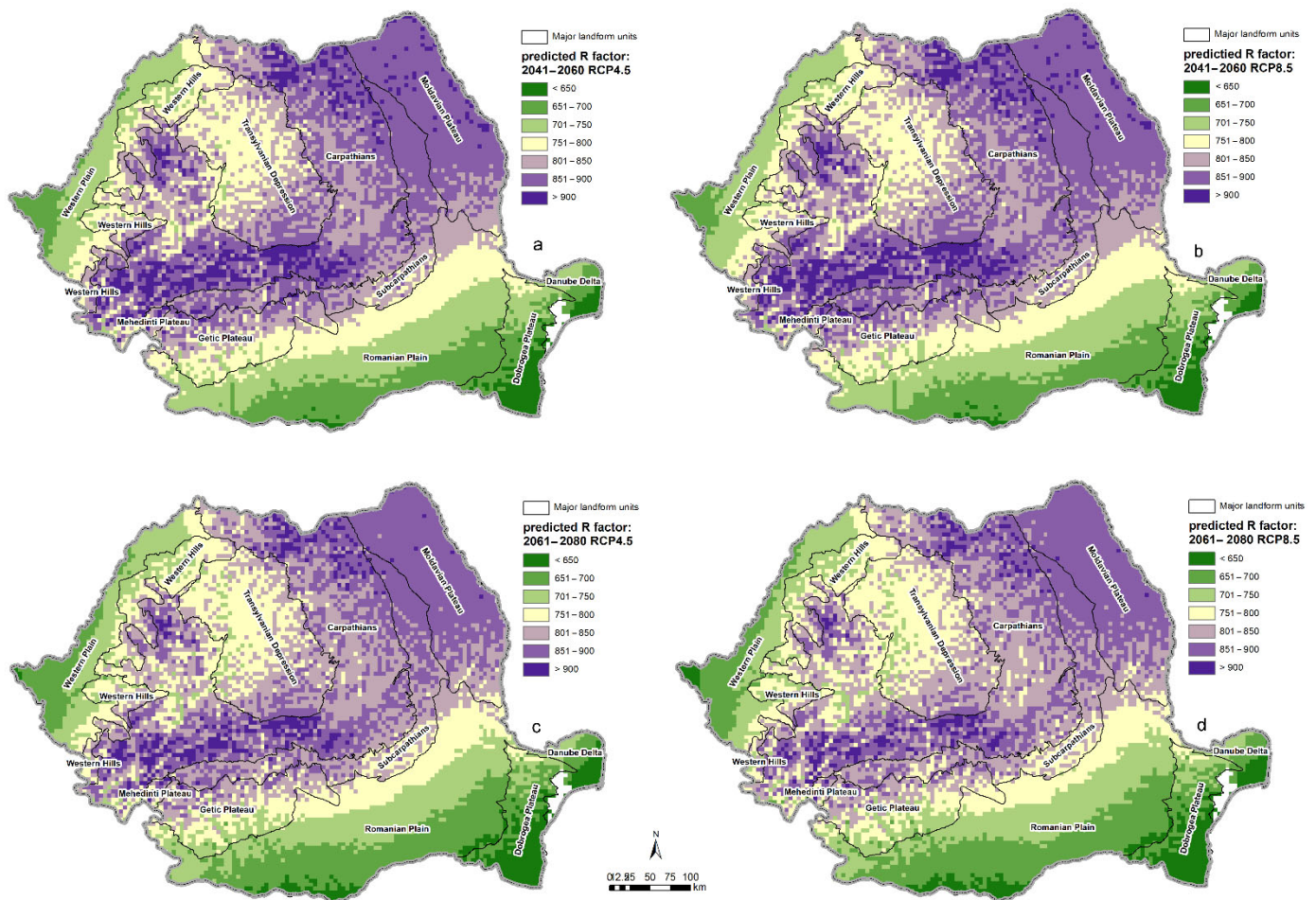
Figure 4. Predicted future rainfall erosivity: (a) 2041–2060 period and RCP 4.5 scenario; (b) 2041–2060 period and RCP 8.5 scenario; (c) 2061–2080 period and RCP 4.5 scenario; (d) 2061–2080 period and RCP 8.5 scenario.
