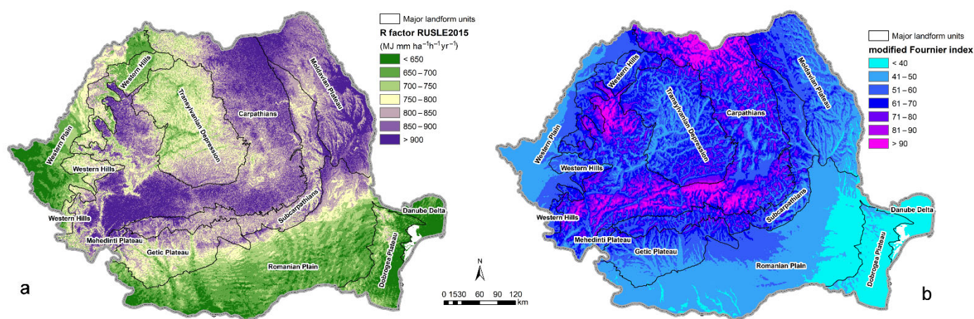
Figure 2. RUSLE 2015 R factor (a) and the modified Fournier index (b) for the current climate.
