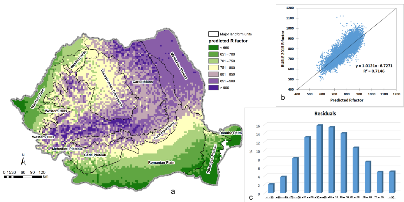
Figure 3. Estimated current R factor at 5 × 5 km resolution based on the non-parametric regression model using LN (MFI), X and Y coordinates as predictor variables: (a) spatial distribution; (b) predicted vs. actual R factor values; (c) distribution of regression residuals.
