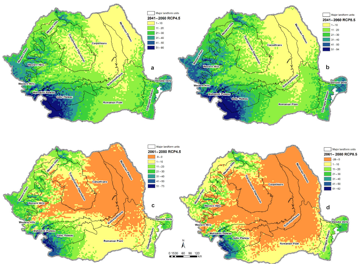
Figure 5. Differences between future and current rainfall erosivity: (a) 2041–2060 period and RCP 4.5 scenario; (b) 2041–2060 period and RCP 8.5 scenario; (c) 2061–2080 period and RCP 4.5 scenario; (d) 2061–2080 period and RCP 8.5 scenario.
