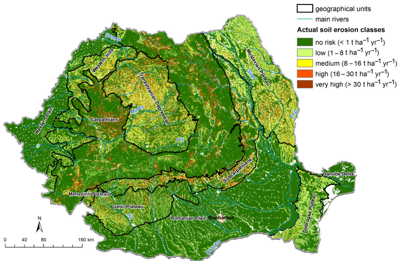
Figure 1. Actual rill and interrill soil erosion map of Romania (Reprinted with permission from [19]. 2019, Soil Use and Management Journal).
