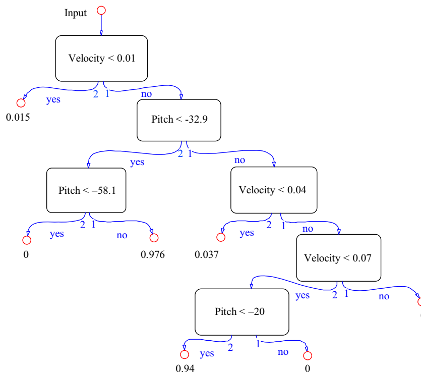
Fig. 8 – Classification tree based on training set with data from 6 individual nodes. At the terminal nodes, an inactive mode is represented by 0 and an active mode is represented by 1.
