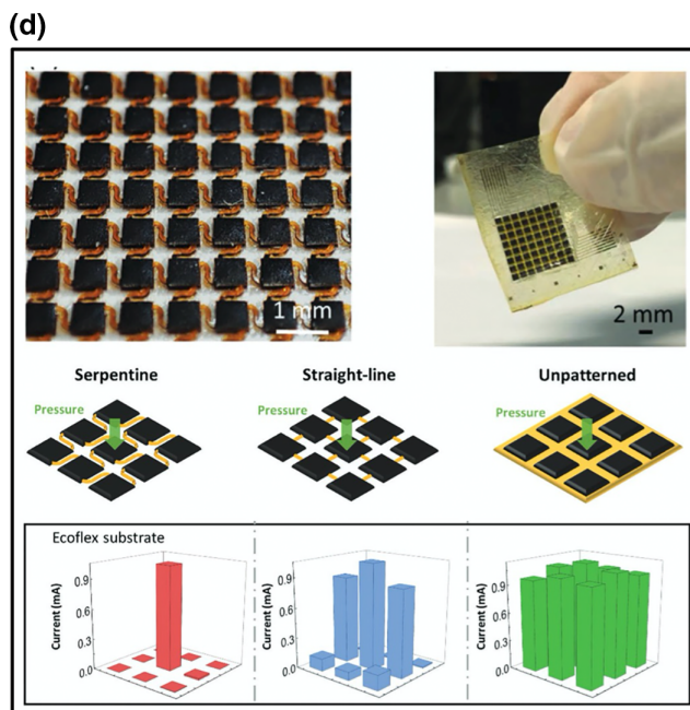
FIGURE 7 Examples of transparent, wireless communication-enabled, and high-density array integrated sensors (a) Transparent triboelectric pressure sensor using a hydrogel triboelectric layer. Reprinted with permission from Pu et al., 2017. Copyright 2017 American Association for the Advancement of Science. (b) RFID-based capacitive pressure sensor for wireless sensing of internal pressures. Reprinted with permission from Lu et al., 2020. Copyright 2020 Wiley-VCH GmbH. (c) High-density transistor array integrated with tactile sensors. Reprinted with permission from Wang, Xu, et al., 2018. Copyright 2018 Macmillan Publishers Limited. (d) Laser-manufactured high-density pressure sensor array with crosstalk minimization through serpentine interconnects. Reprinted with permission from Li et al., 2022. Copyright 2022 Wiley-VCH GmbH.
