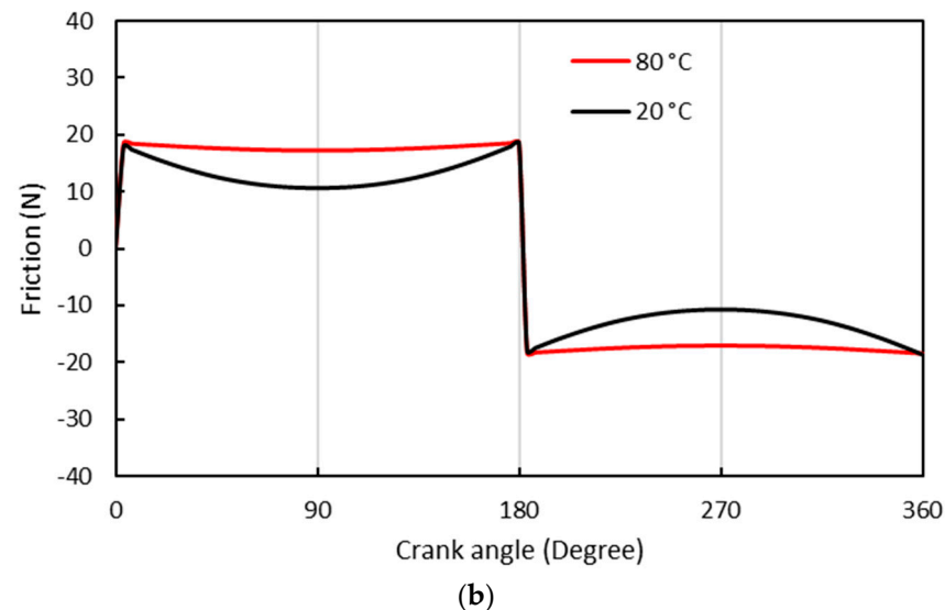
Figure 4. Temperature effect on generated friction for 0W–40 with 2.5% E85 dilution at 600 RPM: (a) experimentally measured, and (b) analytically predicted.
