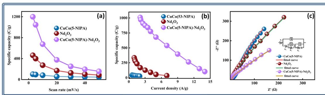
Fig. 5 (a) Specific capacities of CuCo(5-NIPA), \text{Nd}_2\text{O}_3 , and CuCo(5-NIPA)- \text{Nd}_2\text{O}_3 through CV analysis. (b) Specific capacities of CuCo(5-NIPA), \text{Nd}_2\text{O}_3 , and CuCo(5-NIPA)- \text{Nd}_2\text{O}_3 through GCD analysis. (c) Comparison of the electrochemical impedance spectroscopic curves for CuCo(5-NIPA), \text{Nd}_2\text{O}_3 , and CuCo(5-NIPA)- \text{Nd}_2\text{O}_3 along with the fitted curves.
