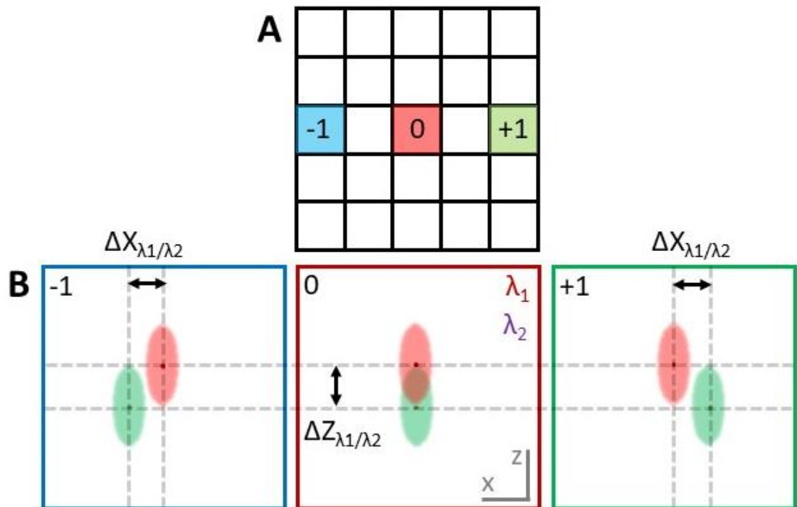
Figure 4.13 Schematic representation of chromatic aberration for a dual beam LSCM set up. A – Raster scanned image field of view. B – Axial chromatic aberration through the optics causes the two laser lines at the centre of the field of view (0) to be shifted in the Z plane by \Delta Z_{\lambda_1/\lambda_2} , while the edges of the field of view (-1, +1) are also shifted in the X dimension by \Delta X_{\lambda_1/\lambda_2} . Adapted from Blanc et al. 17
