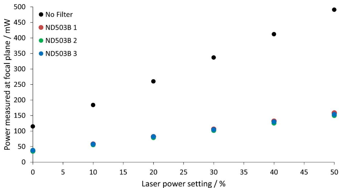
Figure 4.7 Recorded power measurements taken at the focal plane for the multiphoton laser set at 710 nm, in 10% increments, after installation of ND503B.
