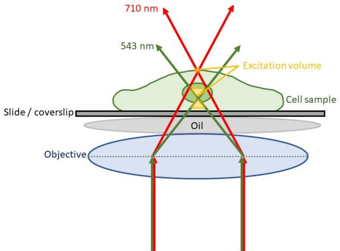
Figure 4.14 Simplified representation of axial chromatic aberration causing 543 and 710 nm laser lines to have differing focal planes.
