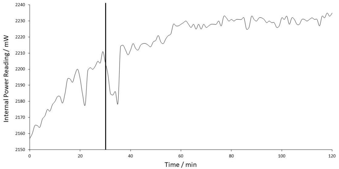
Figure 4.5 Graph logging internal power readings, measured via internal ocean optics HR4000 spectrometer, for the multiphoton laser taken every minute immediately after initialisation. Line added at 30 minutes, where the system reads as fully stabilised.
