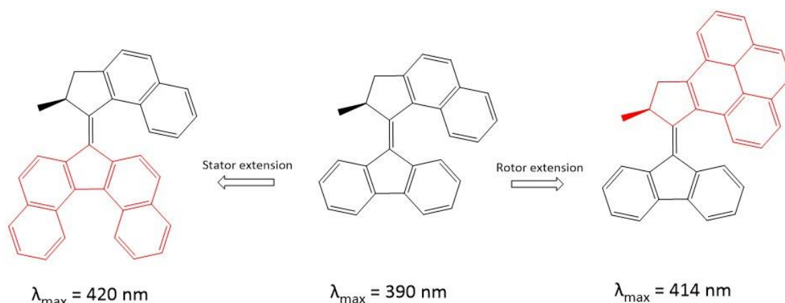
Figure 3.6 Stator (left) and rotor (right) extensions of Feringa motors with their accompanying maximum excitation wavelengths, 420 and 414 nm respectively.
