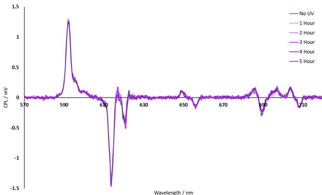
Figure 2.24 Overlaid CPL spectra of Eu(III) complex 1 \Delta when exposed to 355 nm UV for 5 hours, showing no degradation in emission
