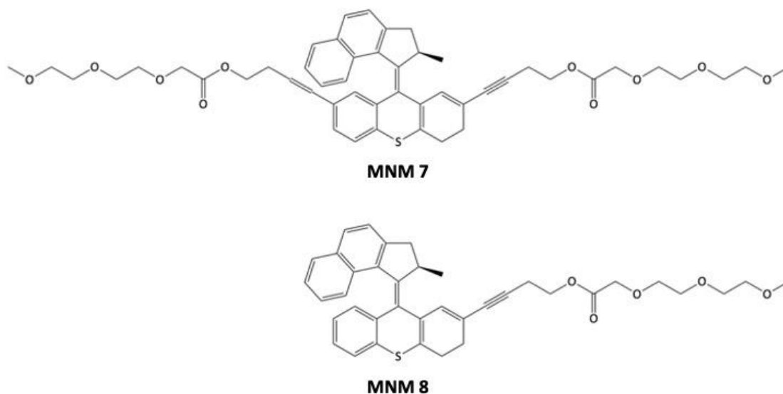
Figure 5.2 Exert from the MNM database showing the chemical structures of two pegylated MNMs used throughout this chapter, dual armed MNM 7 and single arm functionalised MNM 8 .
