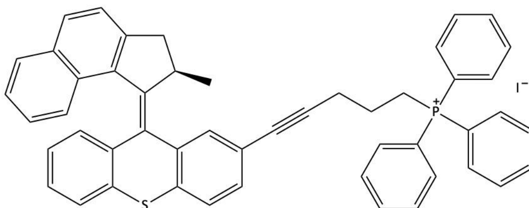
Figure 5.31 Chemical structure of MNM 10 .
