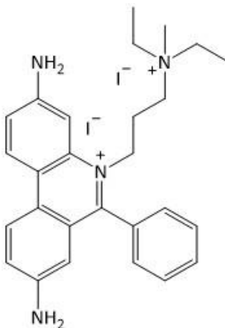
Figure 5.8 Chemical structure of Propidium iodide.
