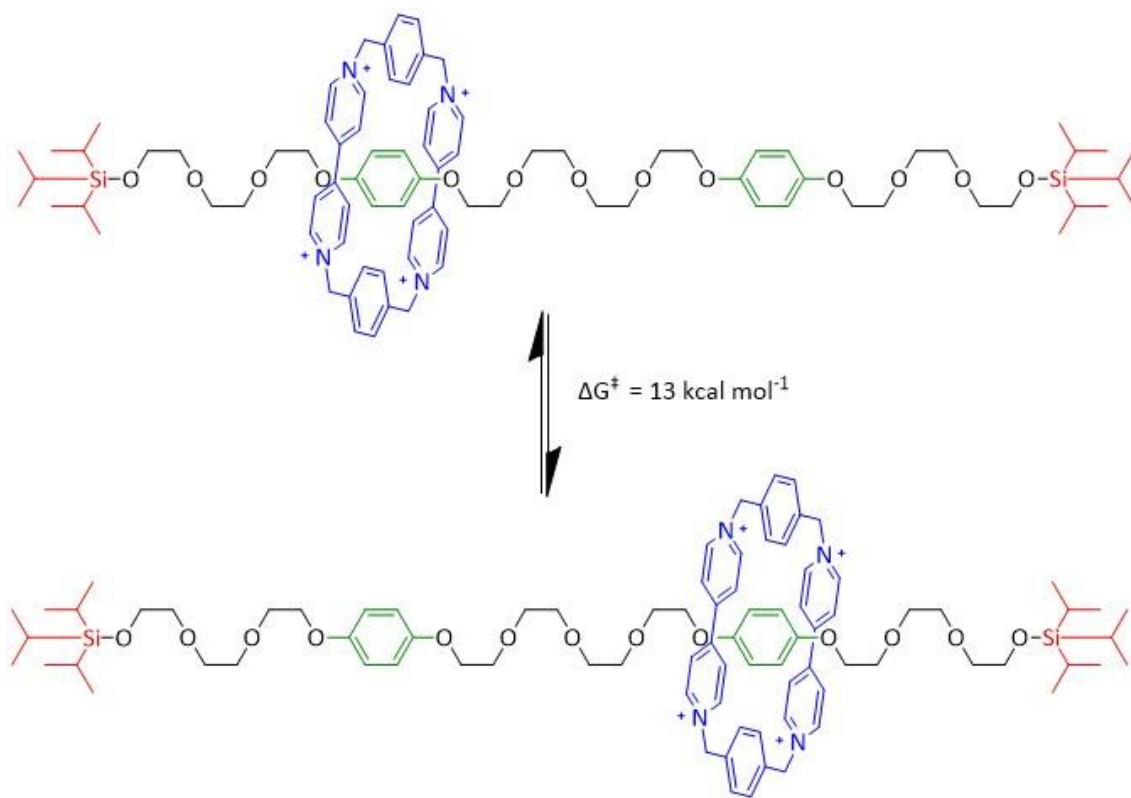
Figure 1.9 Structure and site resonance of the first synthesised degenerate molecular shuttle. The bipyridinium-based cyclophane macrocycle resonates between each 1,4-dioxybenzene site at a rate of about 2000 \text{ s}^{-1} at ambient temperature 49 Again, bulky stopper groups are illustrated in red and the macrocycle is illustrated in blue, while the coordination sites have been coloured green.
