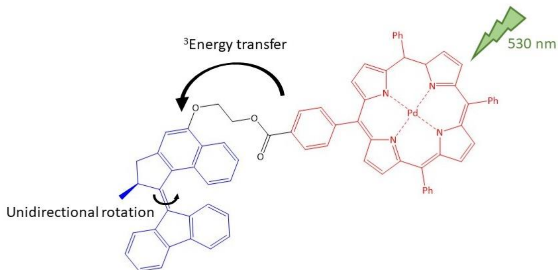
Figure 3.4 Structure and photosensitised activation process for PdTPP (red) functionalised Feringa molecular motor (blue). Adapted from Clossen et al. 5
