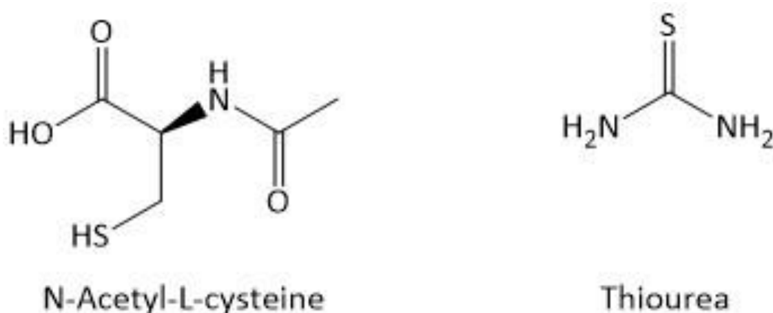
Figure 2.10 Structures of common ROS scavenging species NAC and TU.
