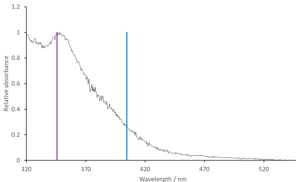
Figure 3.18 UV-Vis absorbance spectrum of MNM 3 in DMSO with purple and blue lines indicating 355 and 405 nm absorbance respectively.
