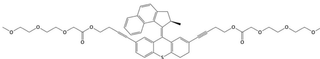
Figure 5.11 Chemical structure of MNM 7 .
