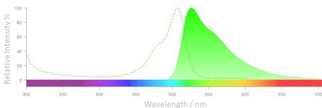
Figure 2.7 Absorption emission spectrum for CellROX™ green reagent.
