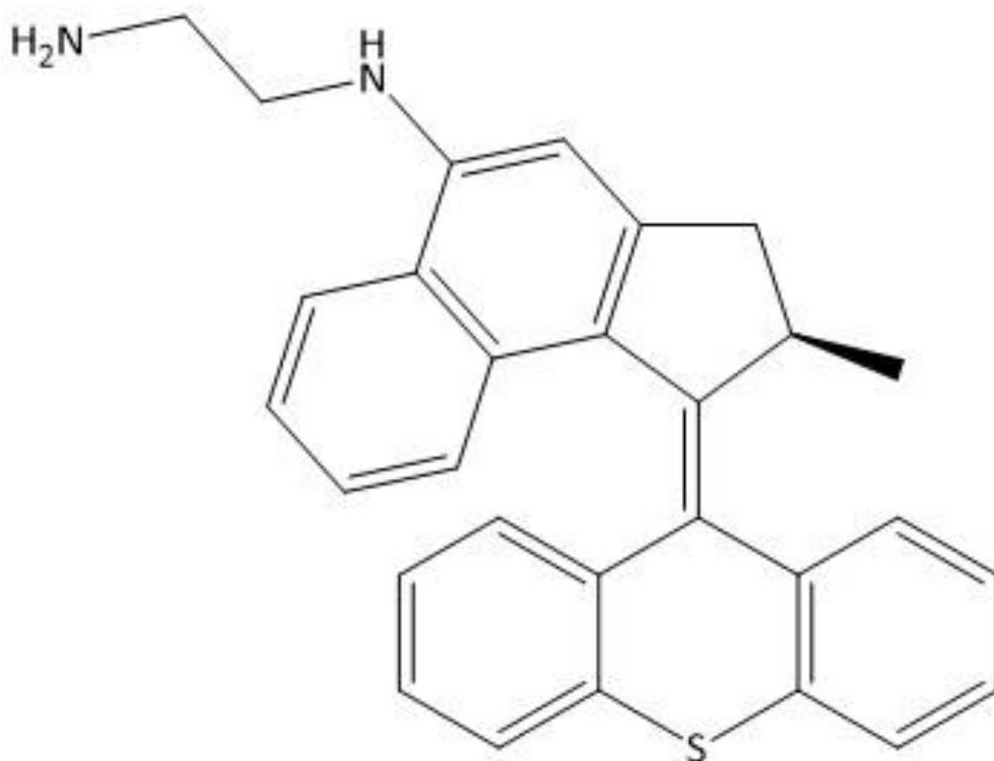
Figure 3.28 Chemical structure of MNM 5 .
