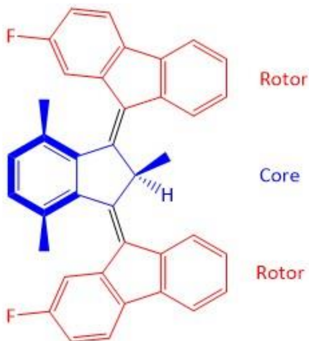
Figure 1.30 Structure of a third generation Ferrocene achiral motor possessing two symmetric overcrowded alkenes and a pseudo-asymmetric carbon atom.
