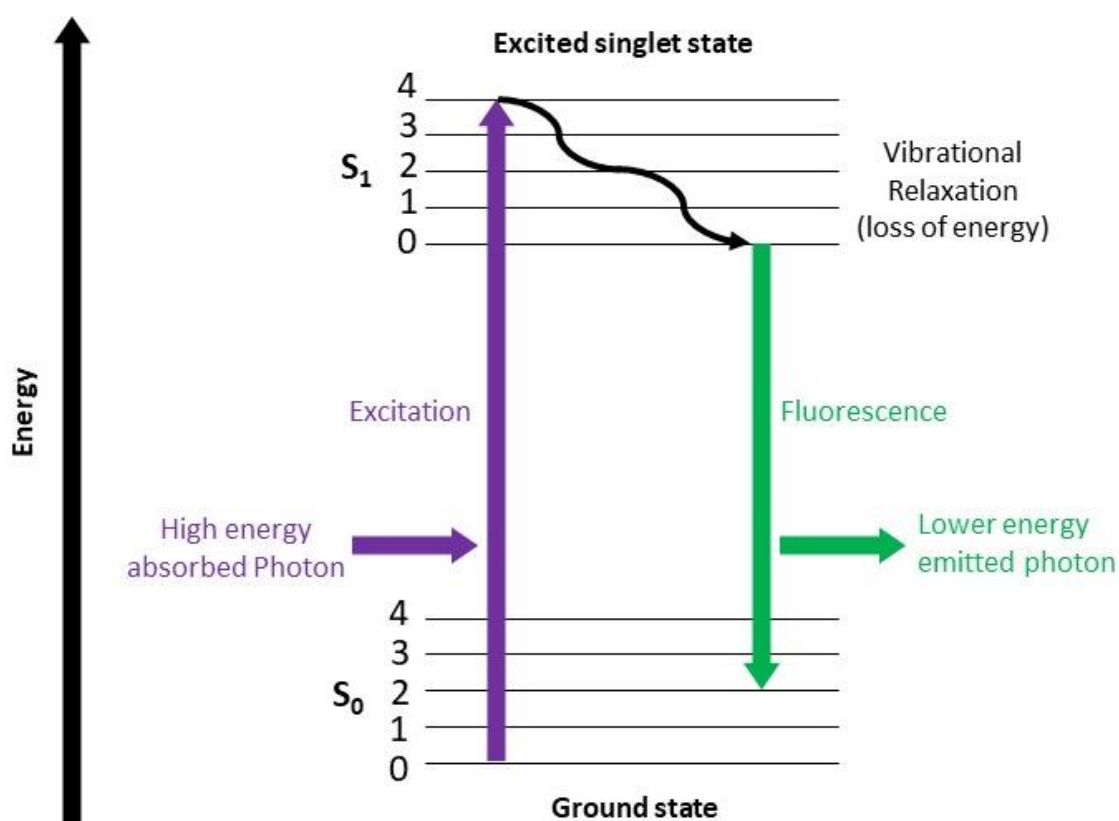
Figure 1.38 Jablonski diagram illustrating the basic processes behind fluorescence.
