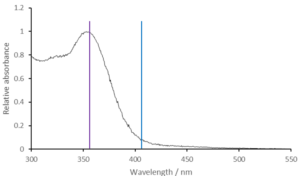
Figure 3.23 UV-Vis absorbance spectrum of MNM 4 in DMSO with purple and blue lines representing 355 and 405 nm absorbance respectively.
