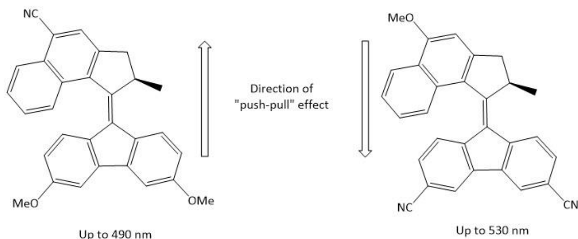
Figure 3.2 Structure of species used to investigate electronic effects on Feringa motor activation wavelengths. Wavelengths stated refer to the low-energy onset of absorption.
