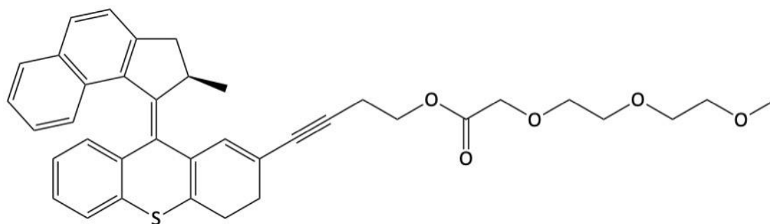
Figure 5.15 Chemical structure of MNM 8 .
