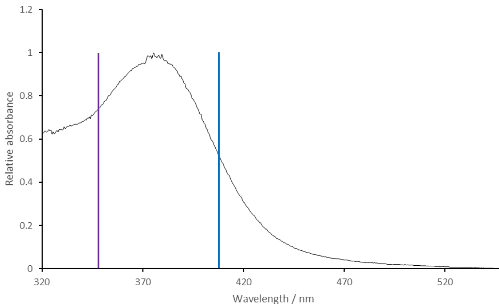
Figure 3.35 UV-Vis absorbance spectrum of MNM 6 in DMSO with purple and blue lines indicating 355 and 405 nm absorbance respectively.
