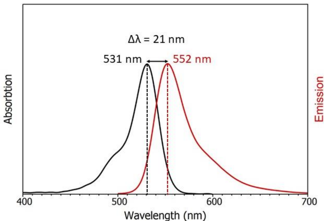
Figure 1.39 Absorption (black) emission (red) spectra for Rhodamine 6G with Stokes shift illustrated. Adapted from Edinburgh Instruments. 101
