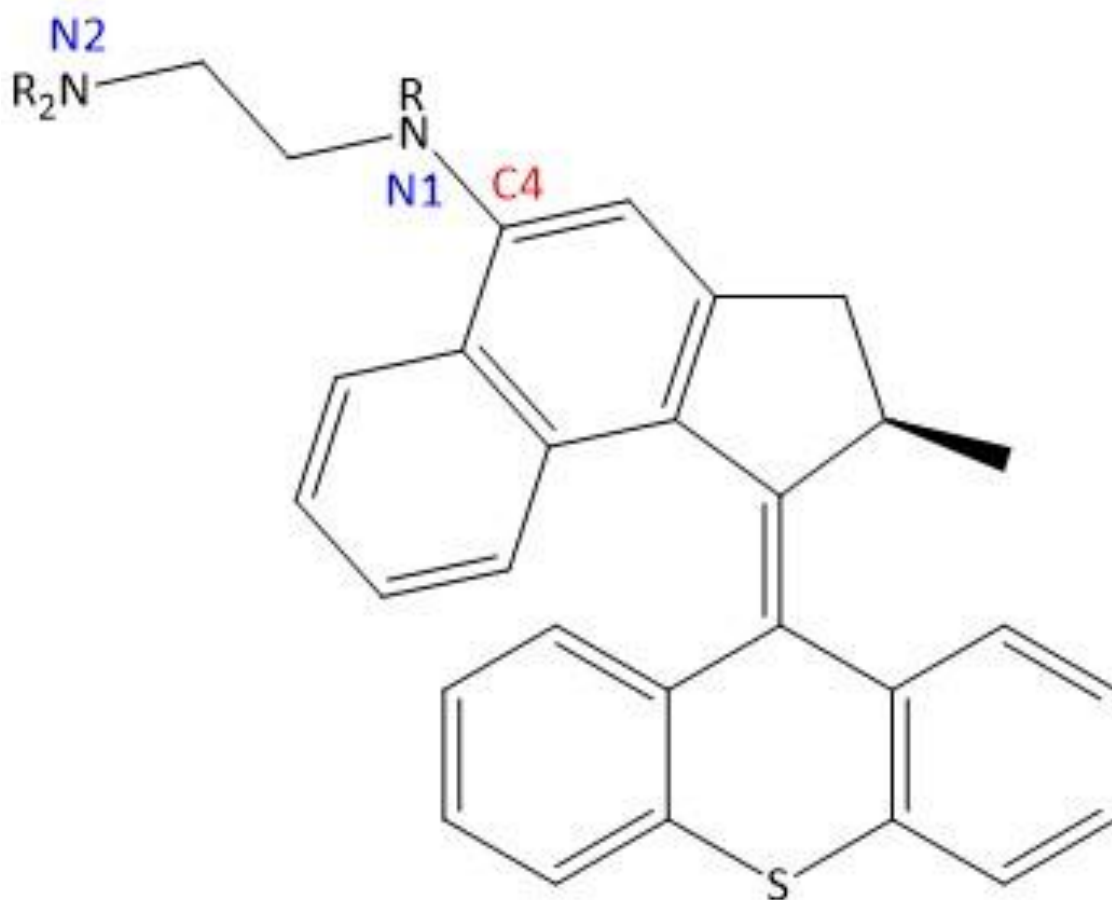
Figure 3.27 General structure for the family of stator "C7" bound diamine MNMs. R = H, Me.
