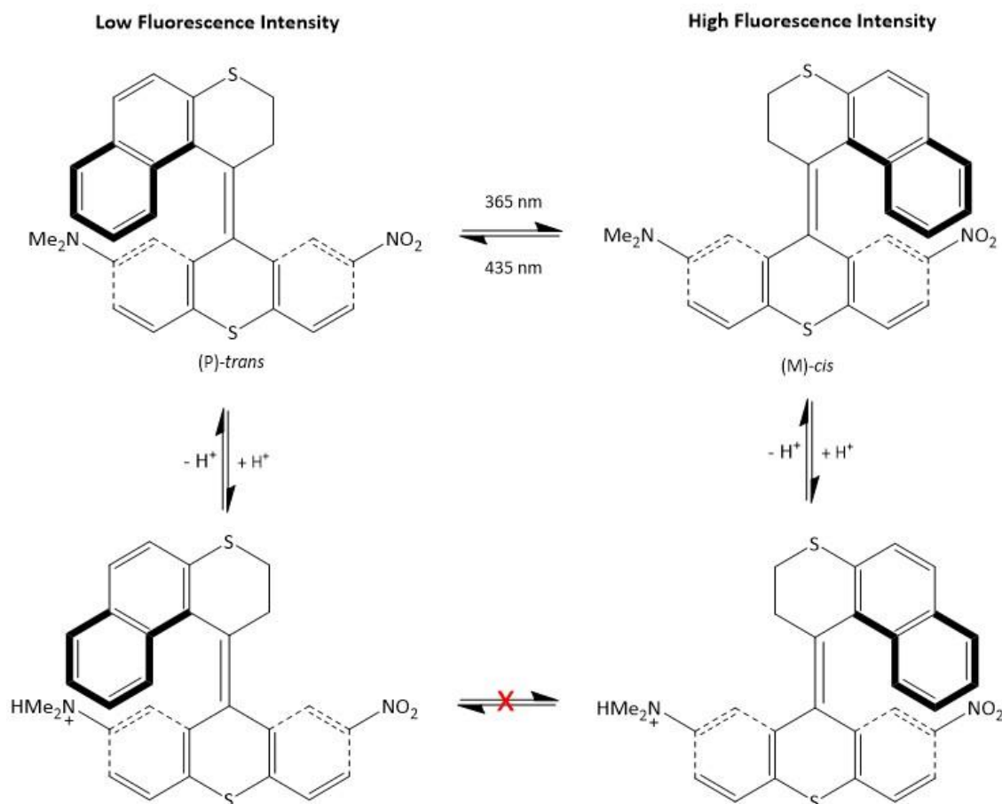
Figure 1.24 Mechanism of dual mode photo-switching fluorescence behaviour of a donor-acceptor molecular switch system. Adapted from Huck et al. 81
