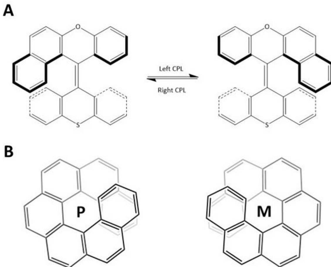
Figure 1.23 A - Switching mechanism of the first reported enantioselective molecular switch. B - Illustration of helical chirality using [7]helicene as an example.
