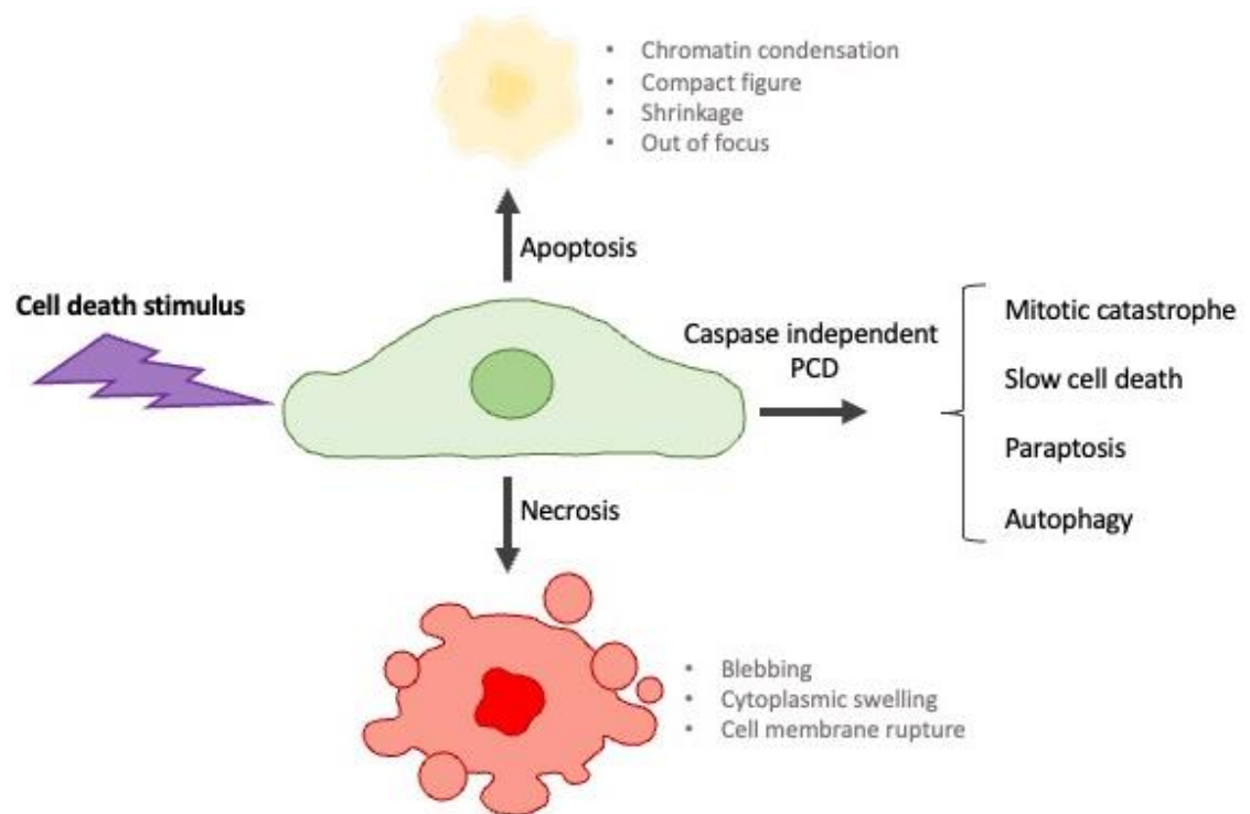
Figure 5.7 Summary of a few key mechanisms of cell death, including several proposed models of caspase independent PCD. Mitotic catastrophe is the default PCD pathway after mitotic failure, slow cell death is a proposed route to describe PCD when caspases are inhibited, paraptosis exhibits cytoplasmic vacuolation and mitochondrial swelling in the absence of caspase activation, and autophagy has been categorised by breakdown of organelles and their subsequent digestion by the cells own lysosomal system. Adapted from Bröker et al. 26
