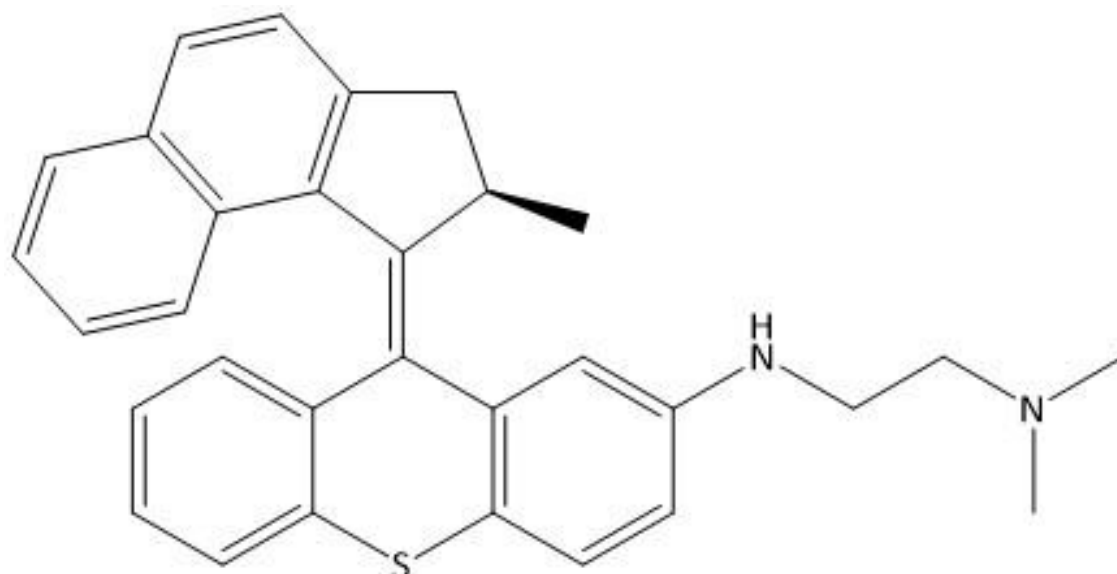
Figure 3.17 Chemical structure of MNM 3.
