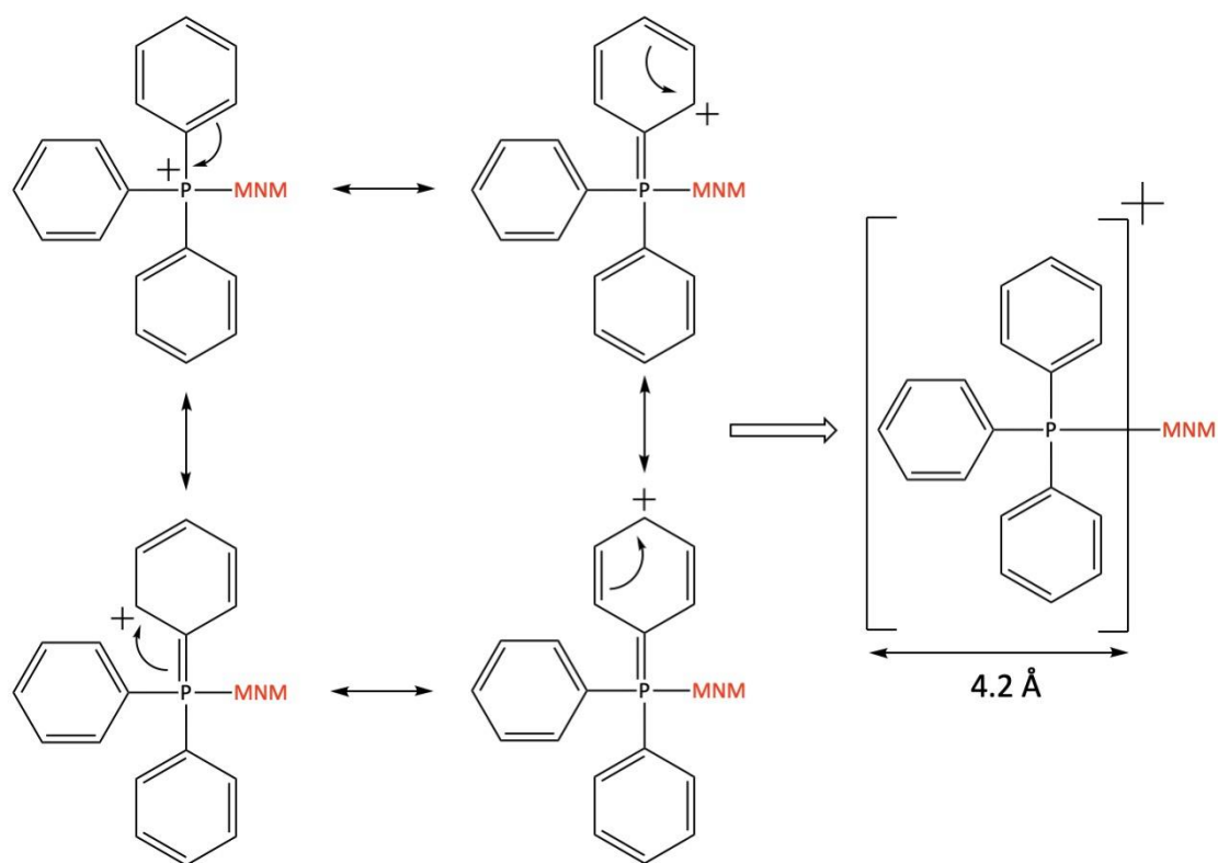
Figure 5.3 Diffusion of positive charge across the TPP + cation via resonance of aryl pi electrons resulting in the observed large ionic radius of 4.2 Å. Adapted from Ross et al. 13
