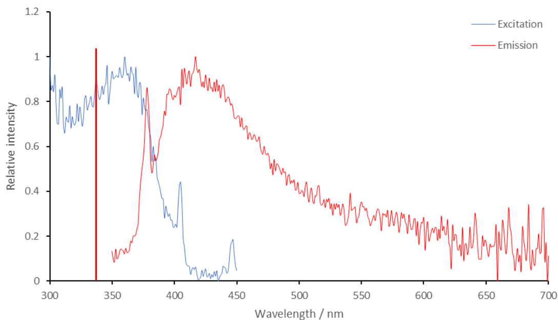
Figure 3.30 Excitation emission spectra for MNM 5 in DMSO. Red line indicates 340 nm excitation.
