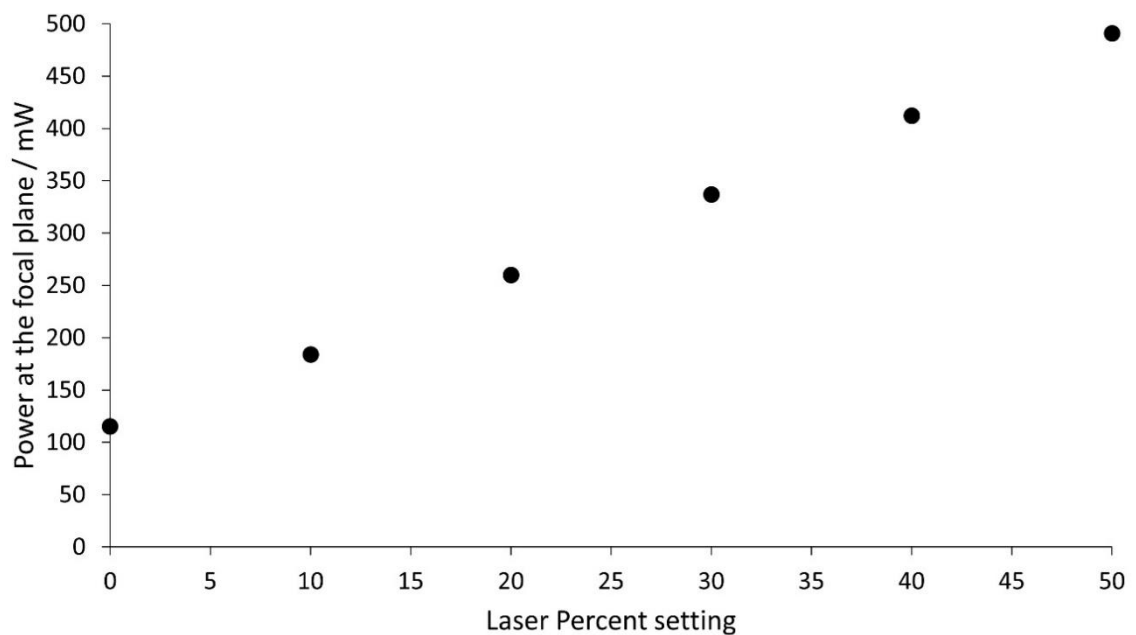
Figure 4.6 Recorded power measurements taken at the focal plane for the multiphoton laser set 710 nm, in 10% increments.
