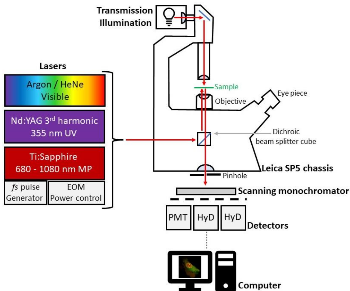
Figure 6.1 Simplified schematic representation of the main hardware components used in the LSCM system used throughout this work.
