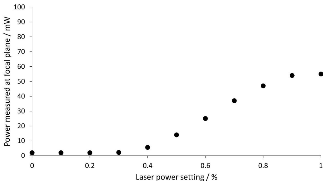
Figure 4.11 Recorded power measurements taken at the focal plane for the multiphoton laser set at 710 nm, in 0.1% increments, after installation of EOM power control.
