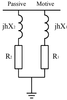
Fig. 6. Load model representation.
