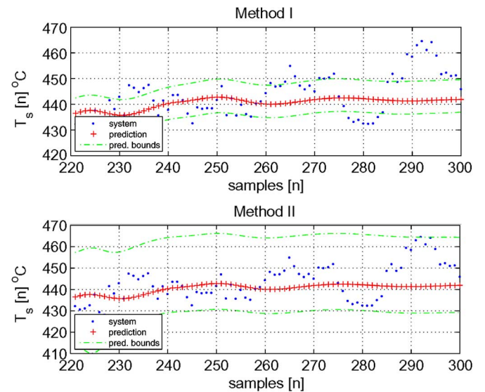
Fig. 10. Plot of predictions using the two statistical based methods for T_s , predicted from sample 220 to sample 300. All predictions are performed from sample 220 and 80 samples into the future (Example 1). The upper plot shows Method I and the lower plot shows Method II.
