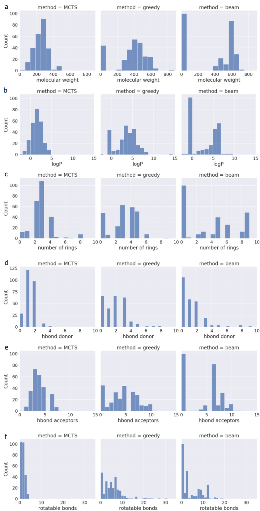
Figure 2. Distribution of properties for the generated molecules across the different decoding algorithms. (a) Molecular weight; (b) water–octanol partition coefficient (logP); (c) the number of rings; (d) the number of H donors; (e) the number of H acceptors; (f) the number of rotatable bonds.
