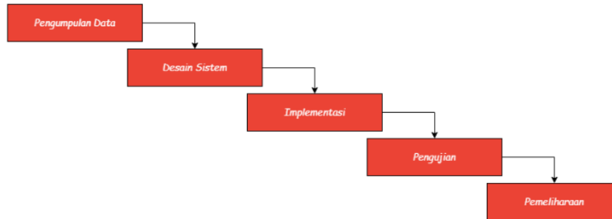
Gambar 1. Metode Waterfall
