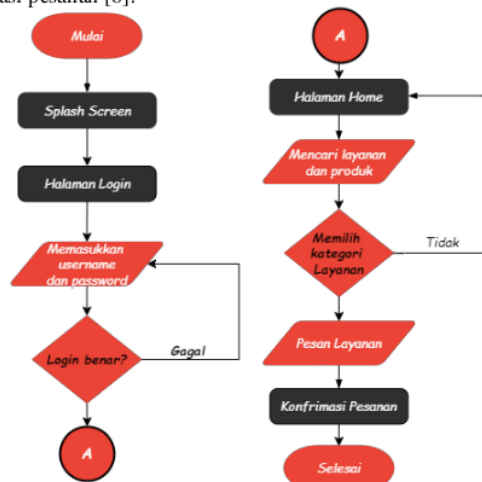
Gambar 2. Flowchart
