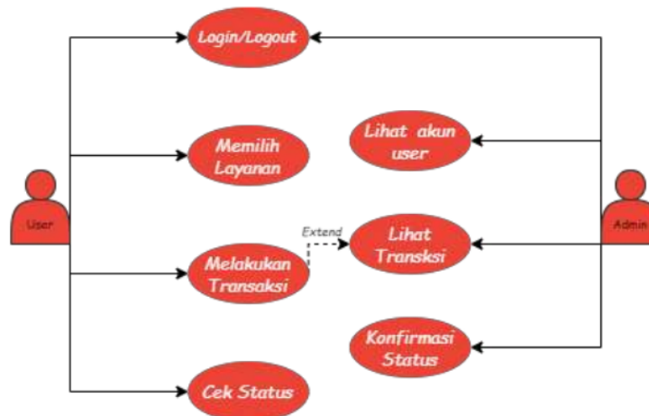
Gambar 3. Usecase Diagram
