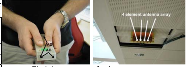
Fig.1 Antenna setup for the measurement setup, left: handheld user device (UD); right: access point device (AP)
