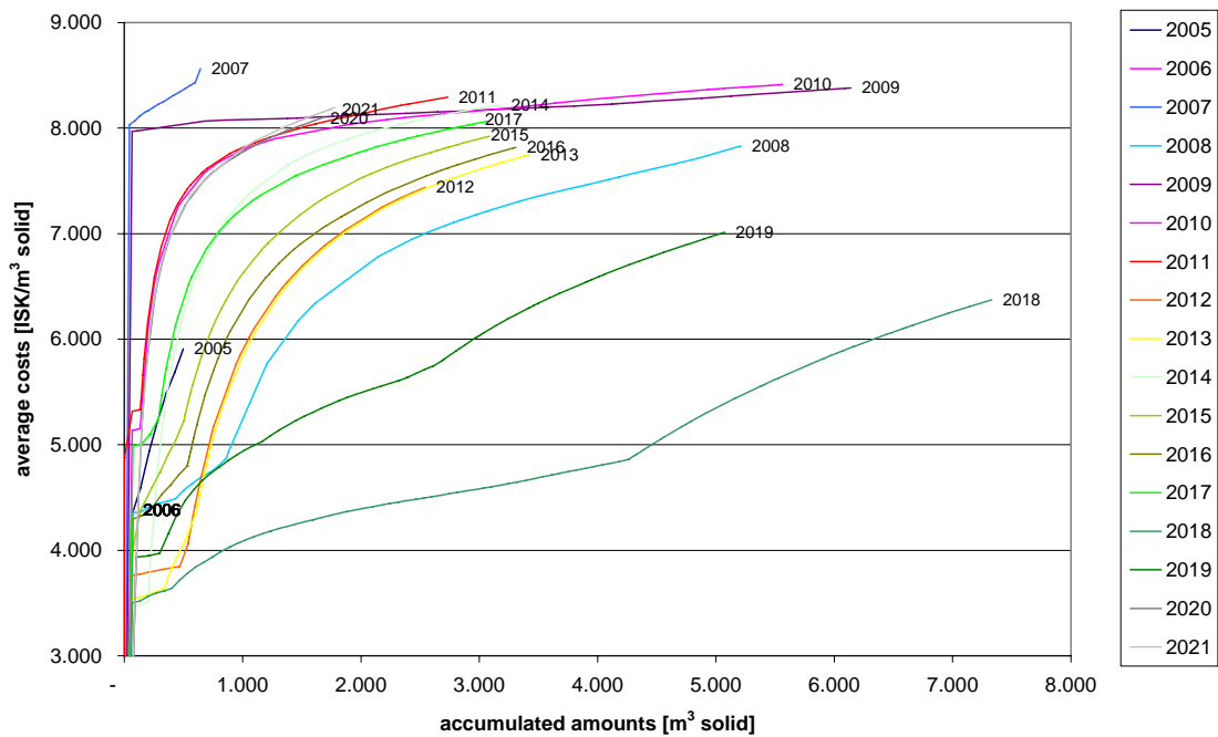
Figure 9: Cost-supply curves for the Hallormsstadur location and for wood resources from Hallormsstadur and Heradsskogar forests. There is a clear tendency of increased costs for increasing amounts. A few years are outliers because of few available resources. A bend in the curves indicates the increase of costs when resources have to be imported from Heradsskogar.
