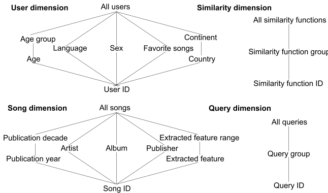
Figure 3: Dimension Hierarchies
