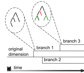
Figure 6: Versioned Hierarchies
