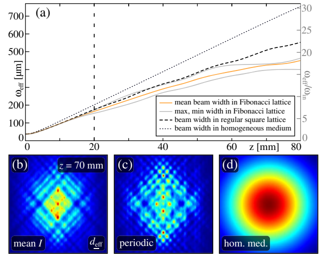
Fig. 7. Comparison of effective beam width development in a Fibonacci lattice against periodic and homogeneous medium cases. (a) Beam widths \omega_{\text{eff}} versus propagation distance z : (orange) mean beam width \omega_{\text{mean}} , and (gray) individual beam width; beam width in (dashed black) a periodic lattice and (dotted black) a homogeneous medium. Dashed vertical line at z = 20 \text{ mm} indicates experimental propagation distance. Intensity distributions at z = 70 \text{ mm} in (b) averaged Fibonacci intensity, (c) periodic square lattice, and (d) homogeneous medium, each for w_0 = 14 \mu\text{m} .
