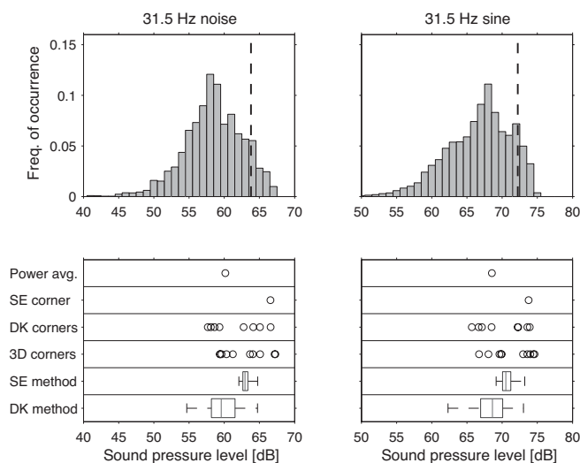
Figure 14 Measurements in living room with 31.5 Hz third-octave-band noise (left) and 31.5 Hz tone (right). Upper frames: Histograms of scannings (dashed line indicates L_{10} , see Discussion); Lower frames: Room power average levels, levels of SE, DK and 3D corners, results of complete Swedish and Danish methods (ranges, lower and upper quartiles, medians from Monte Carlo analyses).
