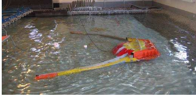
Fig. 4: Testing of 1:50 scale Wave Dragon in Aalborg University wave basin.
