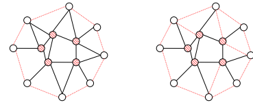
Fig. 1. In this figure, CDS nodes are shown as circles with red line pattern. The left-hand and right-hand figures show the link set (shown as solid black line) used in the routing table calculation in flat and hierarchical routing, respectively.
