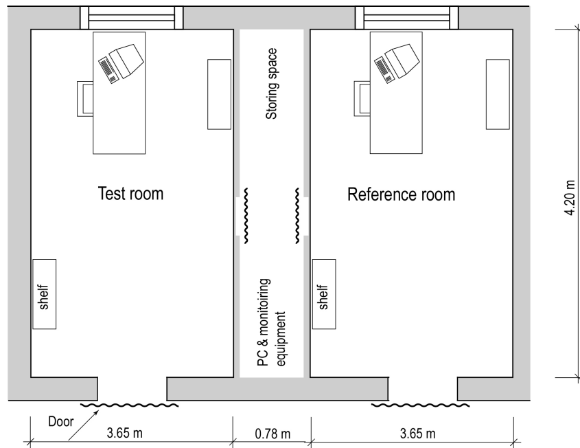
Figure 5: Plan of the experimental rooms in the Daylight Laboratory of ISE Institute showing the Test room and the Reference room, which is furnished, as a typical office room.
