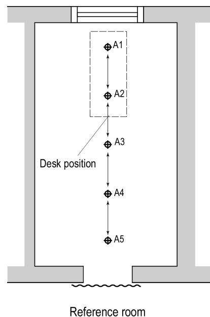
Figure 14 Illuminance ratios that could be studied in the Reference room.
