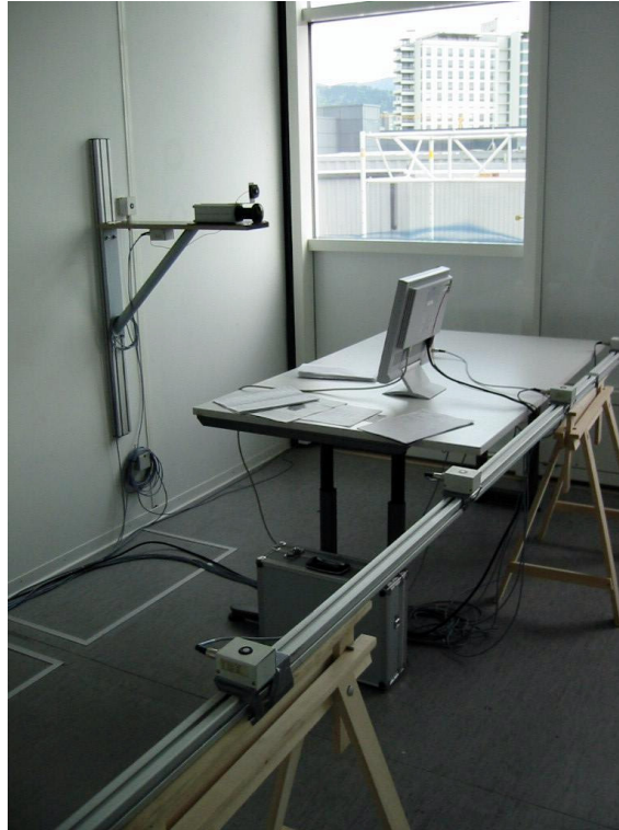
Figure 7: Set up of the monitoring equipment in the Reference room. Interior illuminance on the work plane is measured at 0.85 m from the floor using Hagner lux-meters Model SD2, fixed on metal supports. Mounted on the wall are the CCD camera (LMK98) and the vertical illuminance sensor at the approximate position of the subject's eyes.
