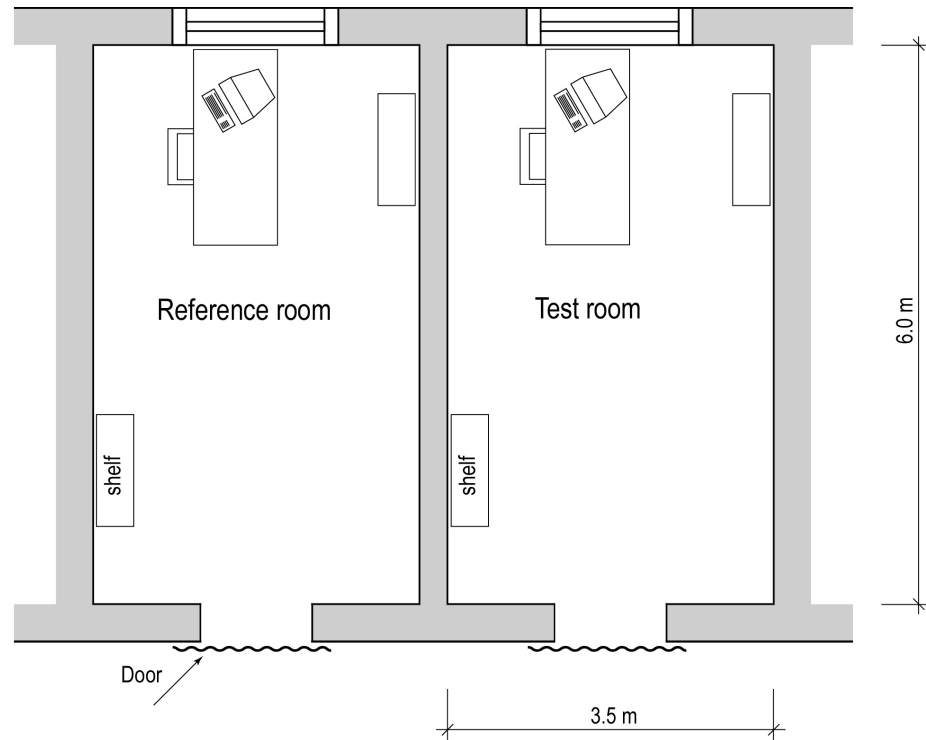
Figure 3 Plan of the experimental rooms in the Daylight Laboratory of DBUR Institute showing the Reference room and the Test room, which is furnished, as a typical office room.
