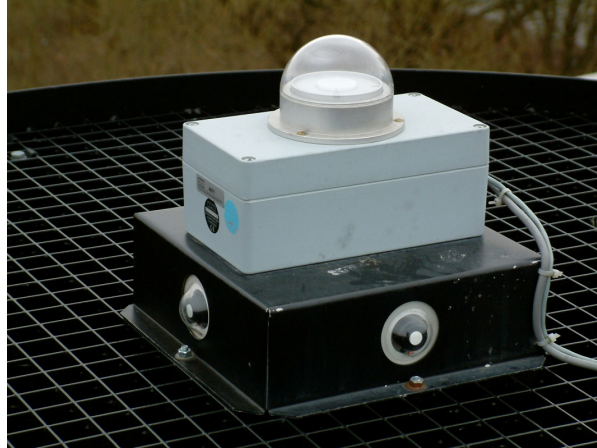
Figure 8 Picture showing the lux meter on the roof at DBUR for recording the global illuminance and the 4 vertical illuminances.
