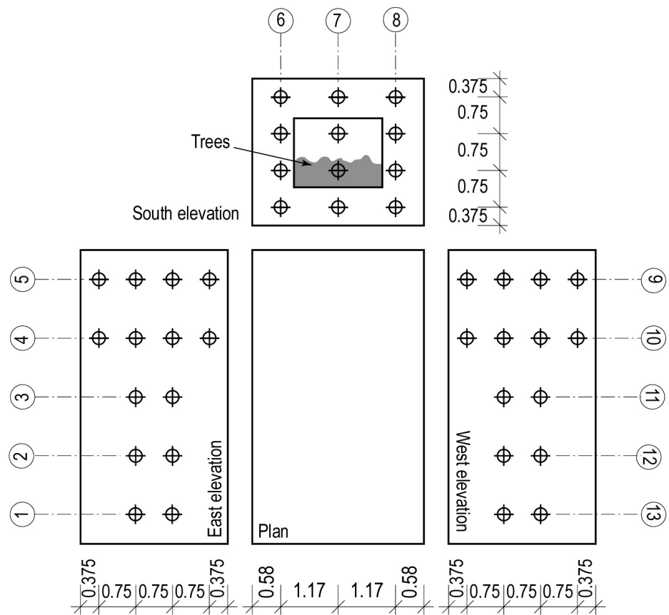
Figure 15 Position of the spots on the walls and windows. Jan – can you help !.
