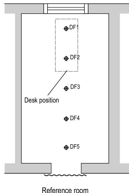
Figure 13 The daylight factor (%) on the work plane that will be studied in the Reference room.
