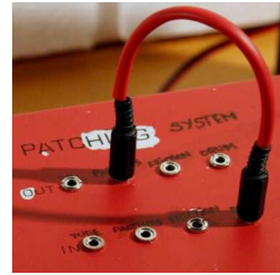
Figure 7: The patching cord system is implemented using 8 mini-jack inputs. They act as on/off switches that establish whether or not they are connected.
