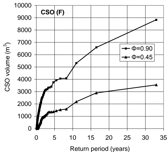
Figure 1. CSO volumes as a function of (average) return period. \phi is the reduction factor.
