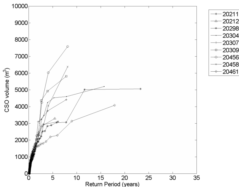
Figure 2. CSO volumes as function of (average) return period. Numbers refer to local rainfall series in the municipality of Aalborg used in MOUSE LTS simulations on the Frejlev catchments.
