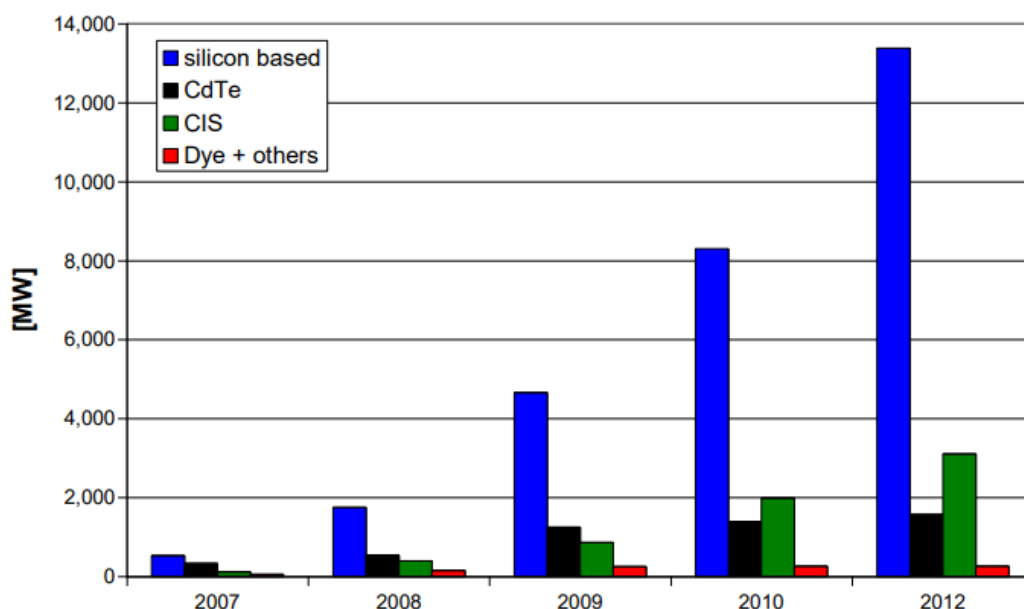
Figure 4. The various technologies' current and projected thin-film photovoltaic production capacity.
