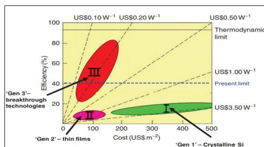
Figure 1. The solar cell landscape, as described by M. Green, demonstrates the aim to create low-cost, high-efficiency Generation III technologies in contrast to Generation II (thin films) and Generation I (silicon).
