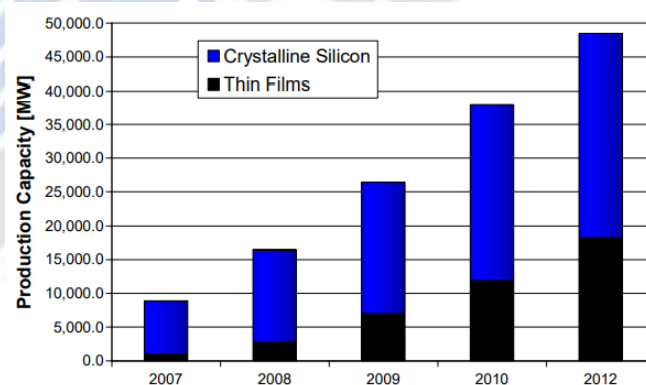
Figure 3. PV, both actual and anticipated Capabilities for producing solar modules based on crystalline silicon and thin film.
