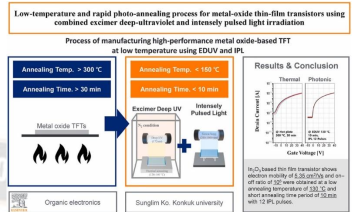
Figure 1 Low-Temperature and rapid photo-annealing process for Metal Oxide Thin-Film Transistors
