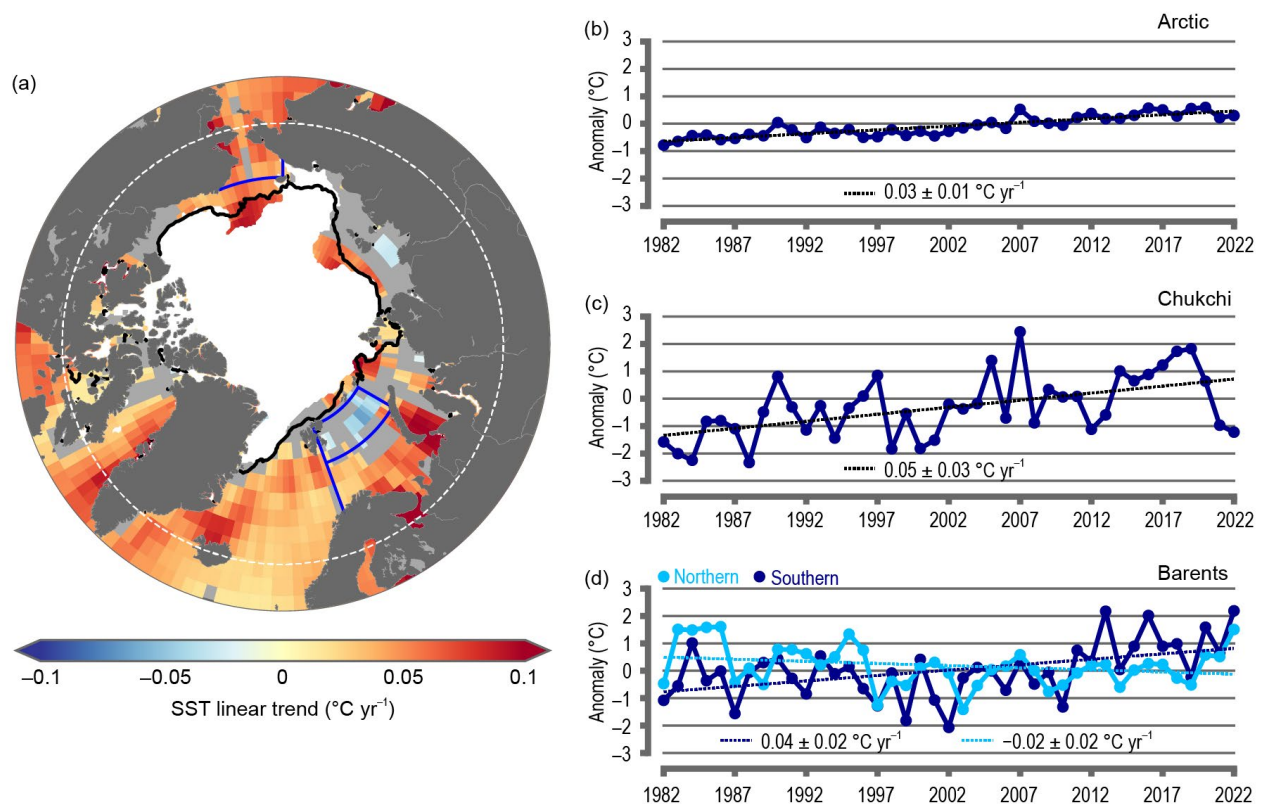
Fig. 5.10. (a) Linear sea-surface temperature (SST) trend ( ^{\circ}\text{C yr}^{-1} ) for Aug of each year from 1982 to 2022. The trend is only shown for values that are statistically significant at the 95% confidence interval; the region is shaded gray otherwise. White shading is the Aug 2022 mean sea-ice extent, and the black line indicates the median ice edge for Aug 1991–2020. (b),(c),(d) Area-averaged SST anomalies ( ^{\circ}\text{C} ) for Aug of each year (1982–2022) relative to the 1991–2020 Aug mean for (b) the entire Arctic Ocean north of 65°N, indicated by the dashed white circle in (a), (c) the Chukchi Sea, and (d) the northern and southern Barents Sea indicated by smaller blue boxes (intersecting with land boundaries) in (a). The dotted lines show the linear SST anomaly trends over the period shown and trends in ^{\circ}\text{C yr}^{-1} (with 95% confidence intervals) are indicated on the plots. See Fig. 5.8 caption for sea ice dataset information.
