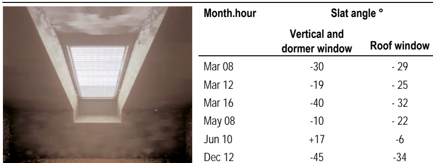
Figure 91. Radiance rendering of the roof window with the Venetian blinds. The table shows the angles of the slats of the Venetian blinds as defined in Figure 88 for each of the simulation hours (cut off angle).
