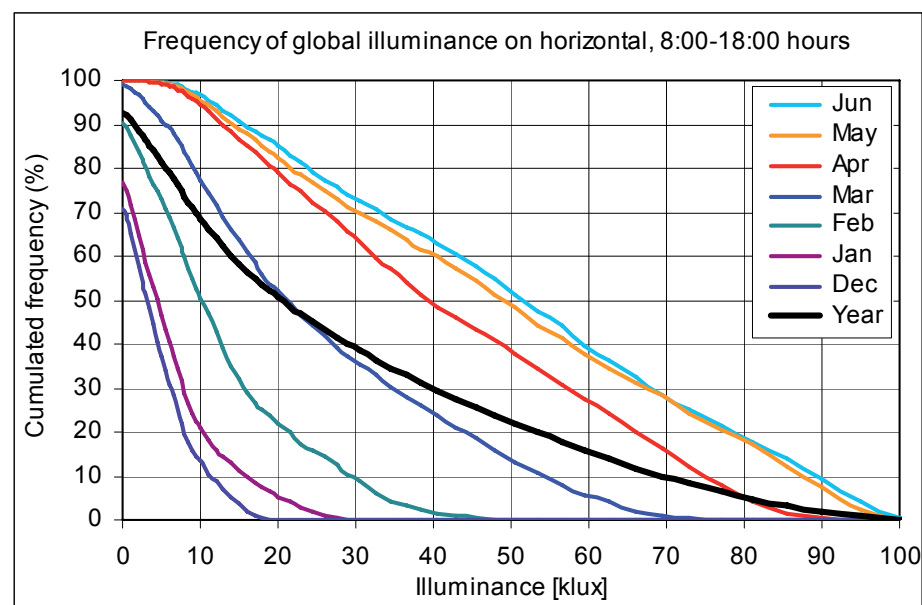
Figure 23. Cumulated frequency of the global illuminance on horizontal for the months December – June within 8:00 – 18:00 hours. The curves show the percentage of hours in each month where the illuminance is above the corresponding value. For example is the illuminance above 30,000 lux in 65 % of the hours in April (66 % of 300 hours, i.e. 195 hours).
