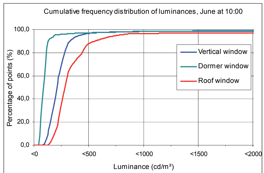
Figure 43. Cumulative frequency distribution of the luminance (cd/m²) for the three window types in the view towards the window under sunny sky in June at 10:00 hours.
