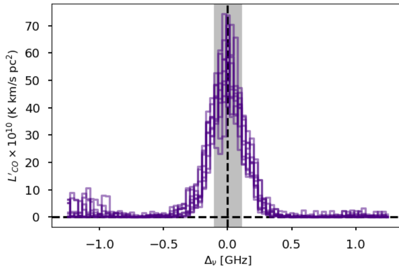
Figure 12. Spectra of simulated stacks, offset to account for the velocity difference between eBOSS-determined redshifts and CO-determined redshifts (z_{\text{CO}} - z_{\text{opt}})/(1 + z_{\text{opt}}) = 0.00408 . Ten different iterations are shown. The fluctuations in the fringes of the spectrum are due to neighbouring objects falling into some cutouts.
