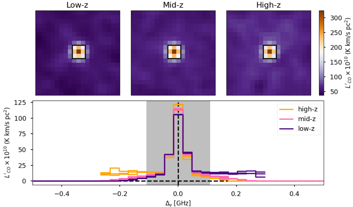
Figure 14. A comparison of constant-luminosity, constant-linewidth simulations at three different redshifts spanning the width of the COMAP data cubes. The spatial distribution of (stacked) emission at each redshift is shown in the top three panels, and the bottom panel shows the spectrum of the stacked cubelets. While the high-redshift stacks are more peaked than the low-redshift stacks, each stack returns the same CO line luminosity. The low-level fringes in the spectra are background emission from objects other than the one being stacked appearing in the spectrum – asymmetries appear due to the low-redshift and high-redshift cutoffs.
