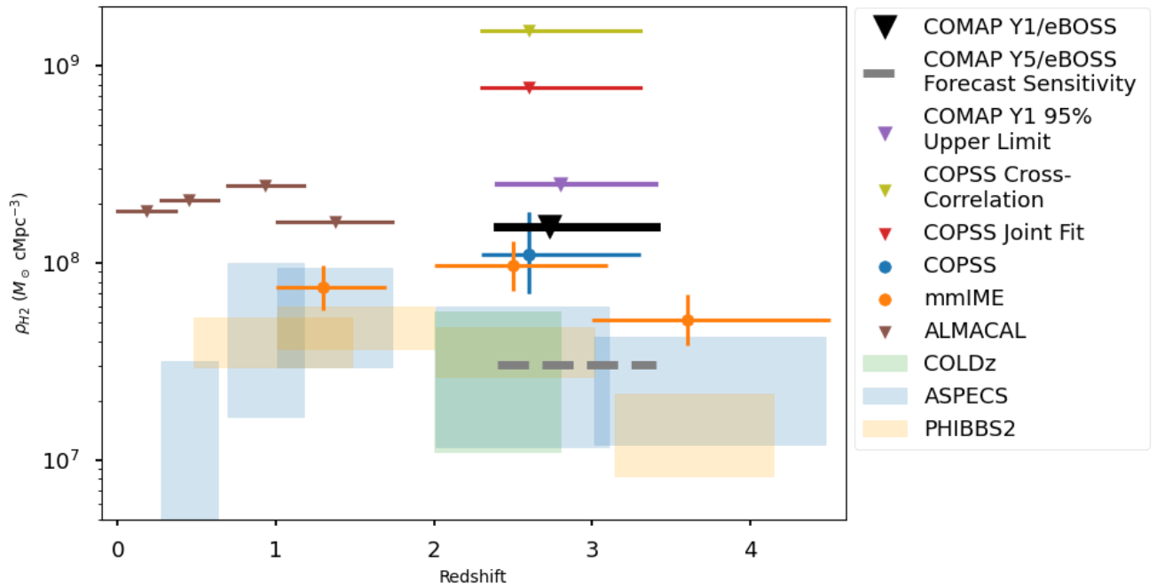
Figure 9. The upper limit on the average molecular gas density determined from the COMAP/eBOSS stack (black line), compared to other \rho_{\text{H}_2} measurements made using different survey techniques. The upper limit from the COMAP Season 1 power spectrum analysis is shown in purple. Also shown is the COPSS LIM survey’s measured value (Keating et al. 2016), as well as upper limits from COPSS joint analyses with galaxy surveys (Keenan et al. 2022). Shaded boxes are measurements made by large-scale traditional surveys COLDz (Riechers et al. 2019), ASPECS (González-López et al. 2019), and PHIBSS2 (Lenkić et al. 2020). We show the forecast 2\sigma sensitivity level of the COMAP survey after five years stacked on eBOSS as a grey upper limit.
