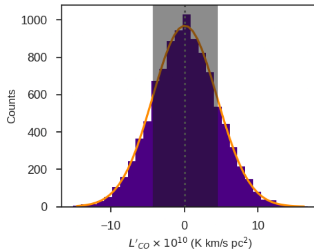
Figure 22. The bootstrapped uncertainty in L'_{CO} for the \text{CN}^- (1-0) stack (see Figure 7).
