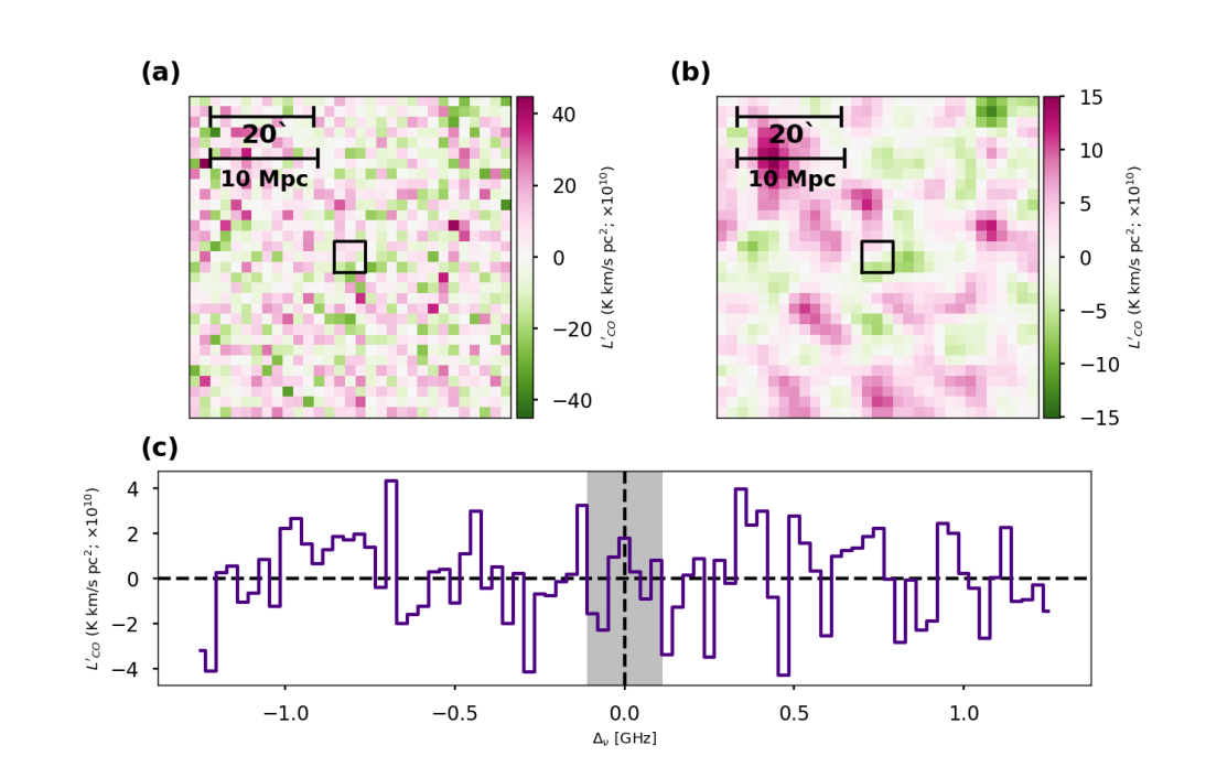
Figure 10. The 3D stack performed on the eBOSS catalog using the ^{12}\text{CO}(1-0) emission wavelength offset by the frequency offset found in individually-detected quasars (see §4.2.3). See Figure 6 for panel descriptions.
