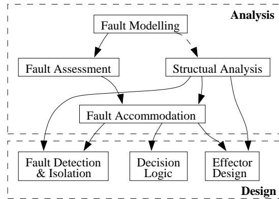
Fig. 2. Systematic fault tolerant control system development approach.
