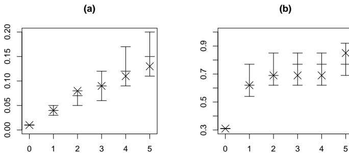
Figure 4.6: Central 95% prediction intervals and medians (indicated by bars) for the rate of Ips spp. colonization over time t = 0, \dots, 5 among those trees that were alive at t = -1 and (a) were not colonized by turpentine beetles ( x_{i,0} = 0 ) or (b) were colonized by turpentine beetles ( x_{i,0} > 0 ). The corresponding observed rate of Ips spp. colonization are indicated by crosses. Note the different scales on the y -axes.
