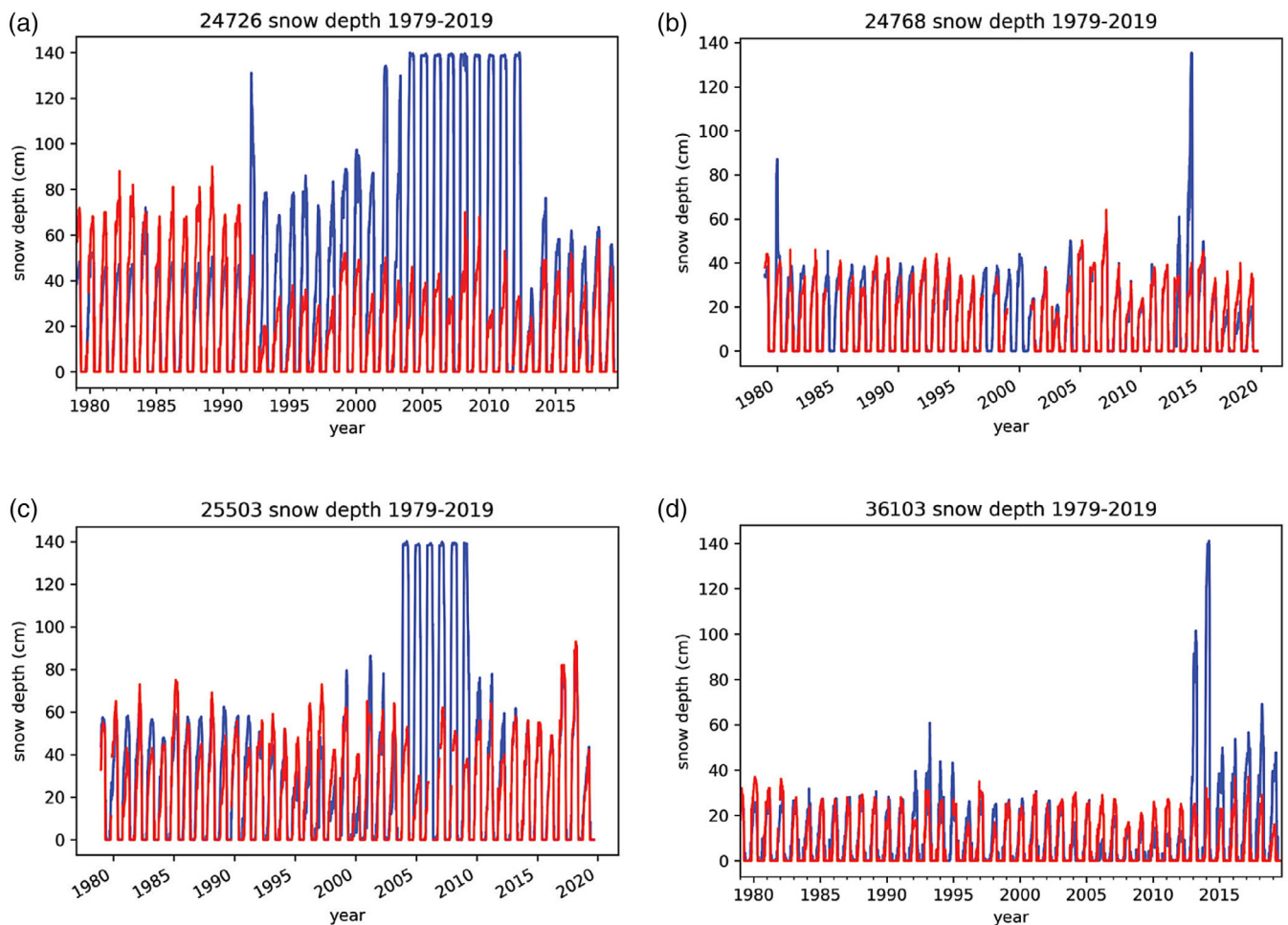
FIGURE 11 ERA-Interim (blue) and meteorological station (red) snow depth (SD) values, 1979–2019, for stations 24726 (a), 24768 (b), 25503 (c) and 36103 (d). Note that station 24768 has no data available in 1984, 1997, 1999 and 2000. [Colour figure can be viewed at wileyonlinelibrary.com ]
