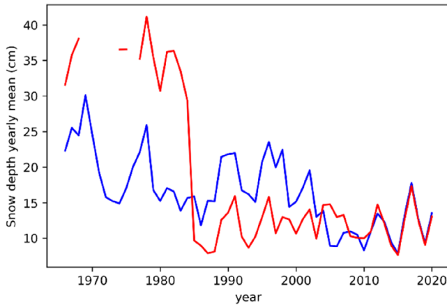
FIGURE 3 The mean yearly snow depth (SD) at station 24371 for the years 1966–2020. The blue and red lines show the ERA5 and station values, respectively. [Colour figure can be viewed at wileyonlinelibrary.com ]
