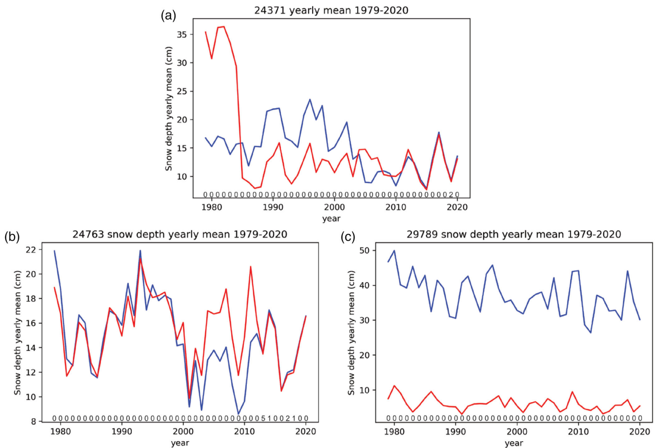
FIGURE 14 ERA5 (blue) and meteorological station (red) snow depth (SD) values per year, 1979–2020, for stations 24371 (a), 24763 (b) and 29789 (c) with the number of assimilations per year. [Colour figure can be viewed at wileyonlinelibrary.com ]
