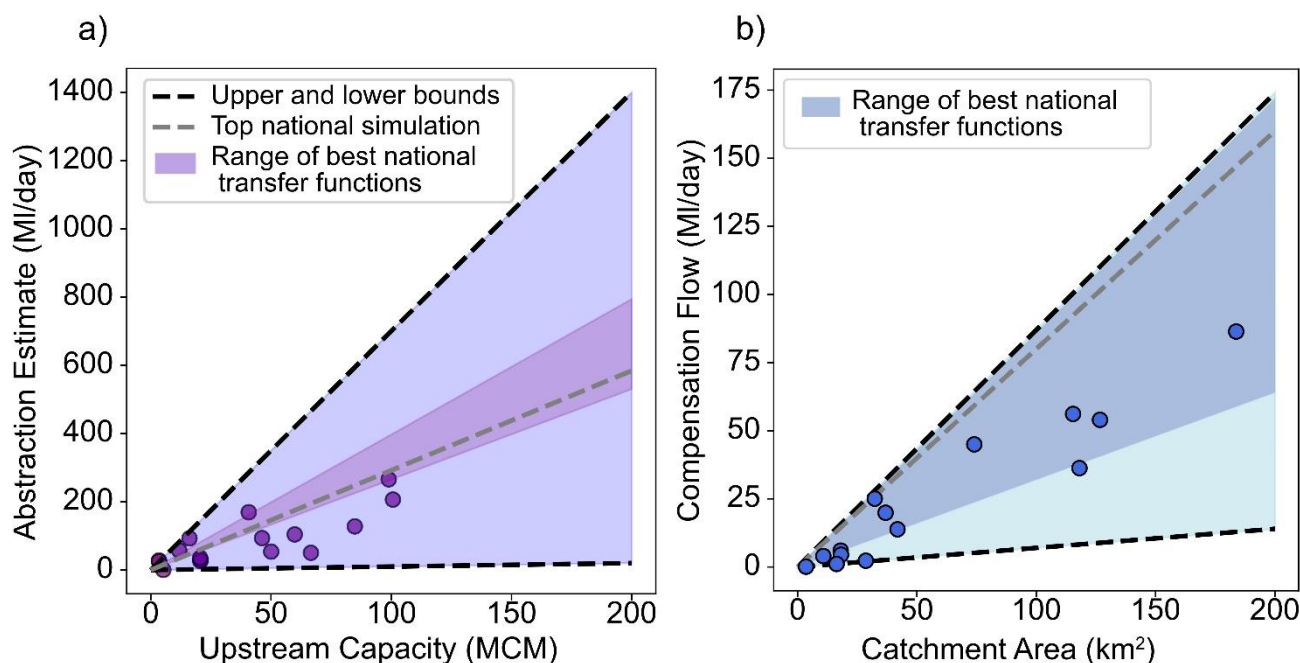
Figure 3. Relationship between (a) reservoir capacity upstream of a gauge and the reservoir abstraction volume (ABS) and 325 (b) catchment area upstream of a gauge and compensation flow (CF). Dots represent data from a sample of catchments where abstractions could be estimated using a water balance hydrological signature and compensation flows could be extracted from Drought Plans, WRMPs and observed downstream flow duration curves (see Section 3.5.1 and Section 1 in Supplementary Material). Grey dashed lines represent the linear transfer functions associated with the best performing simulation from the nationally-consistent calibration, the darker shading represents the spread of the top 5% of nationally-consistent simulations 330 and black dashed lines represent the limits of the transfer function parameters based on the sensitivity of model performance to these parameters (see Table S1 and Section 2 in the Supplementary Material).
