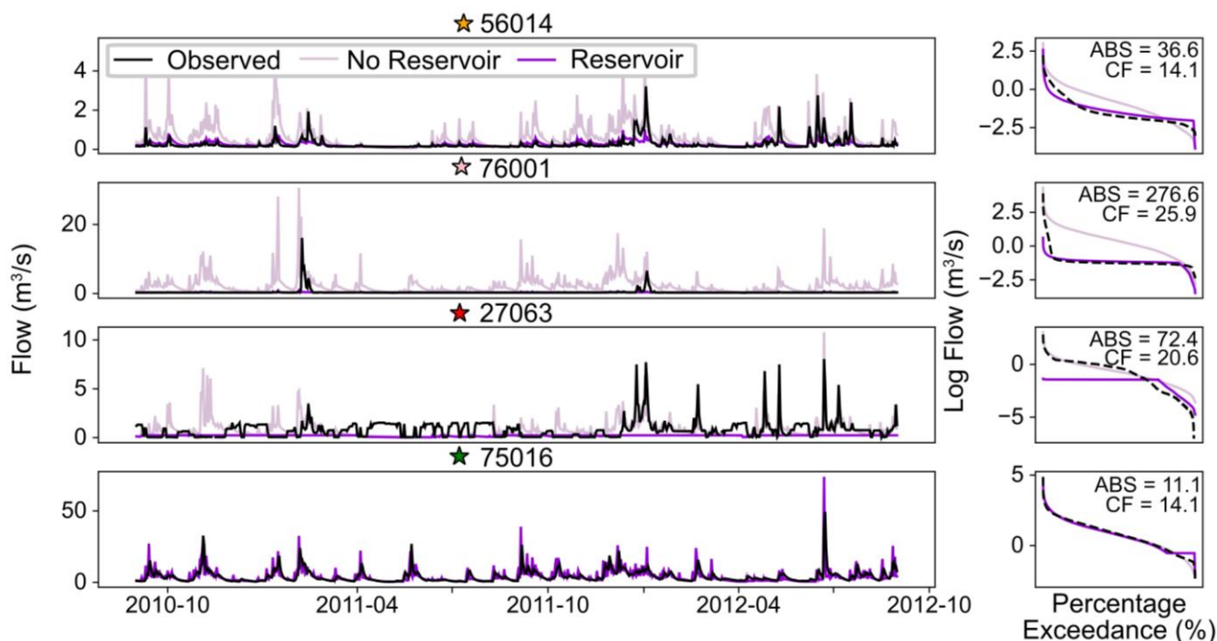
Figure 7. Hydrographs and flow duration curves from best median simulation (nationally-consistent calibration) for selected reservoir catchments. CF and ABS are recorded on each catchments flow duration curve in MI/day.
