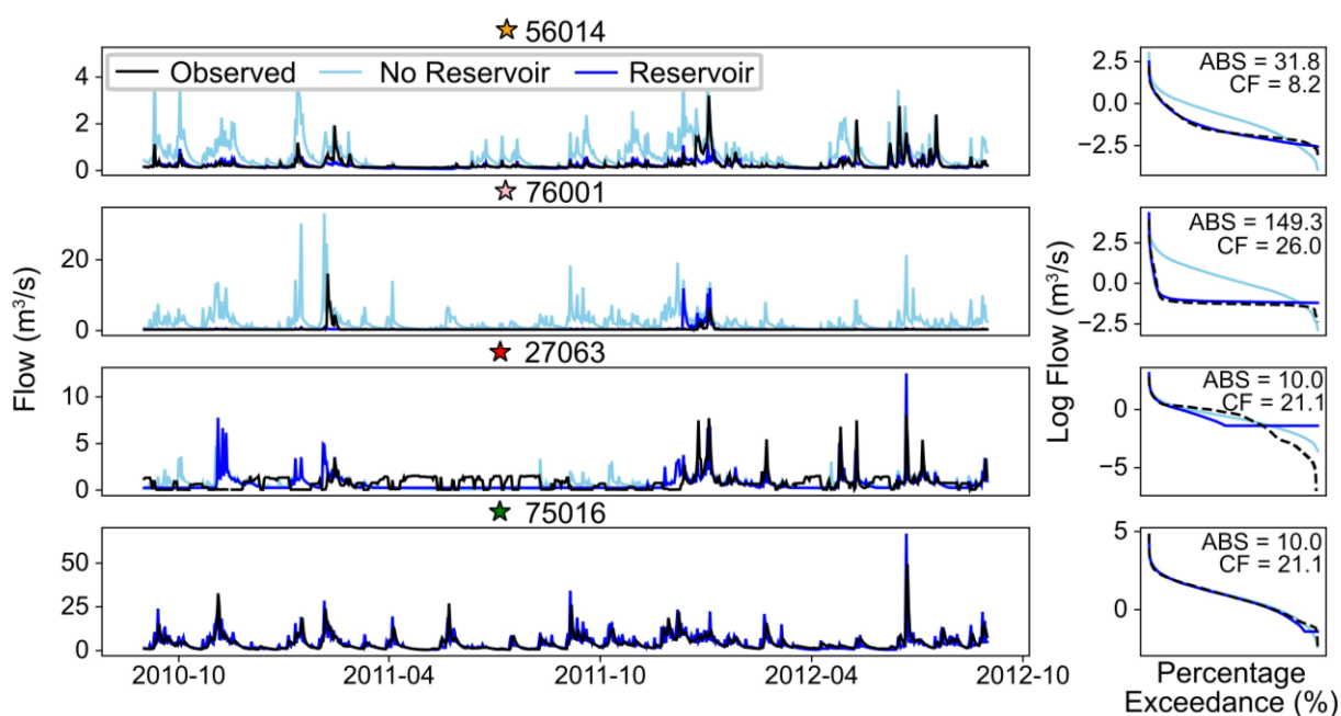
Figure 6. Hydrographs and flow duration curves from the best individual simulations (catchment-by-catchment) for selected reservoir catchments. CF and ABS are recorded on each catchments flow duration curve in MI/day.
