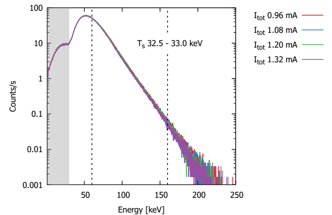
Fig. 8. The bremsstrahlung spectra (counts/second) of the CUBE-ECR ion source with total extracted currents of 0.96 – 1.32 mA with 250 W microwave power at 10.96 GHz frequency. The total current was varied by changing the argon gas feed rate into the ion source.
