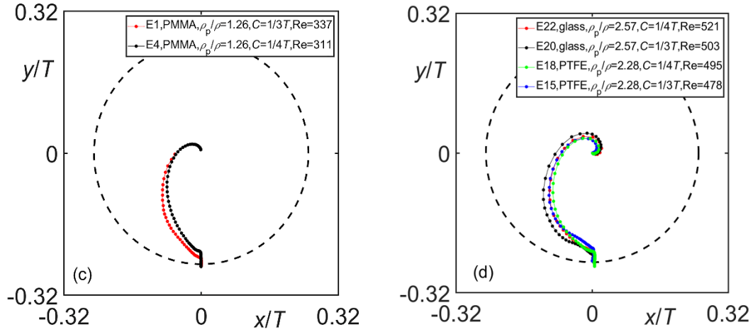
FIGURE 3 Trajectories of particles rolling on the tank bottom. (a) Effect of Re at C = 1/4T ; (b) effect of particle density at C = 1/4T ; (c-d) effect of impeller off-bottom clearance.
