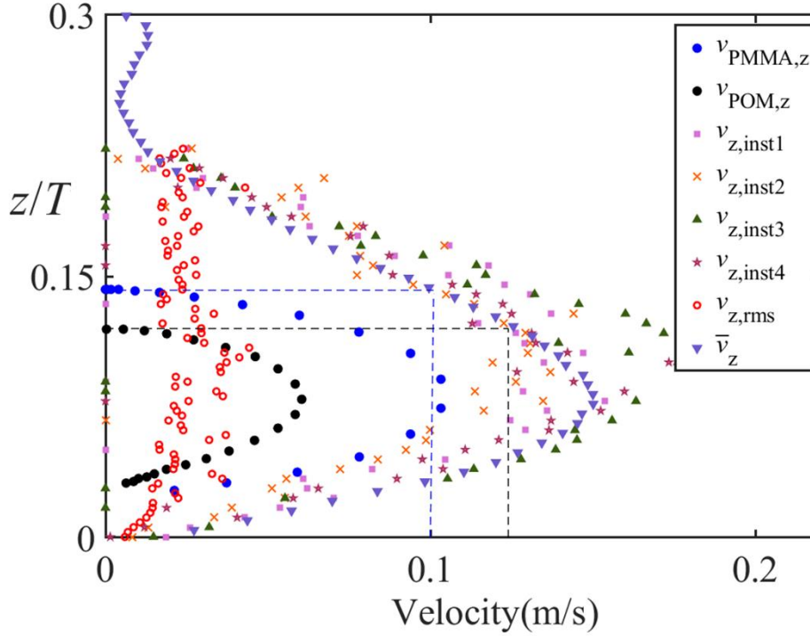
FIGURE 10 Profiles of velocity component in z direction, including PMMA particle velocity component at Re=383 , POM particle velocity component at Re=375 , four instantaneous liquid velocity component at Re=383 , rms of liquid velocity fluctuation component at Re=383 , and phase-averaged liquid velocity component at Re=383 . The dashed lines show that at the stagnation points of the PMMA and POM particles, the average liquid velocity component in z direction are about 0.10 m/s and 0.12 m/s, respectively. C=1/3T , x/T=0 .
