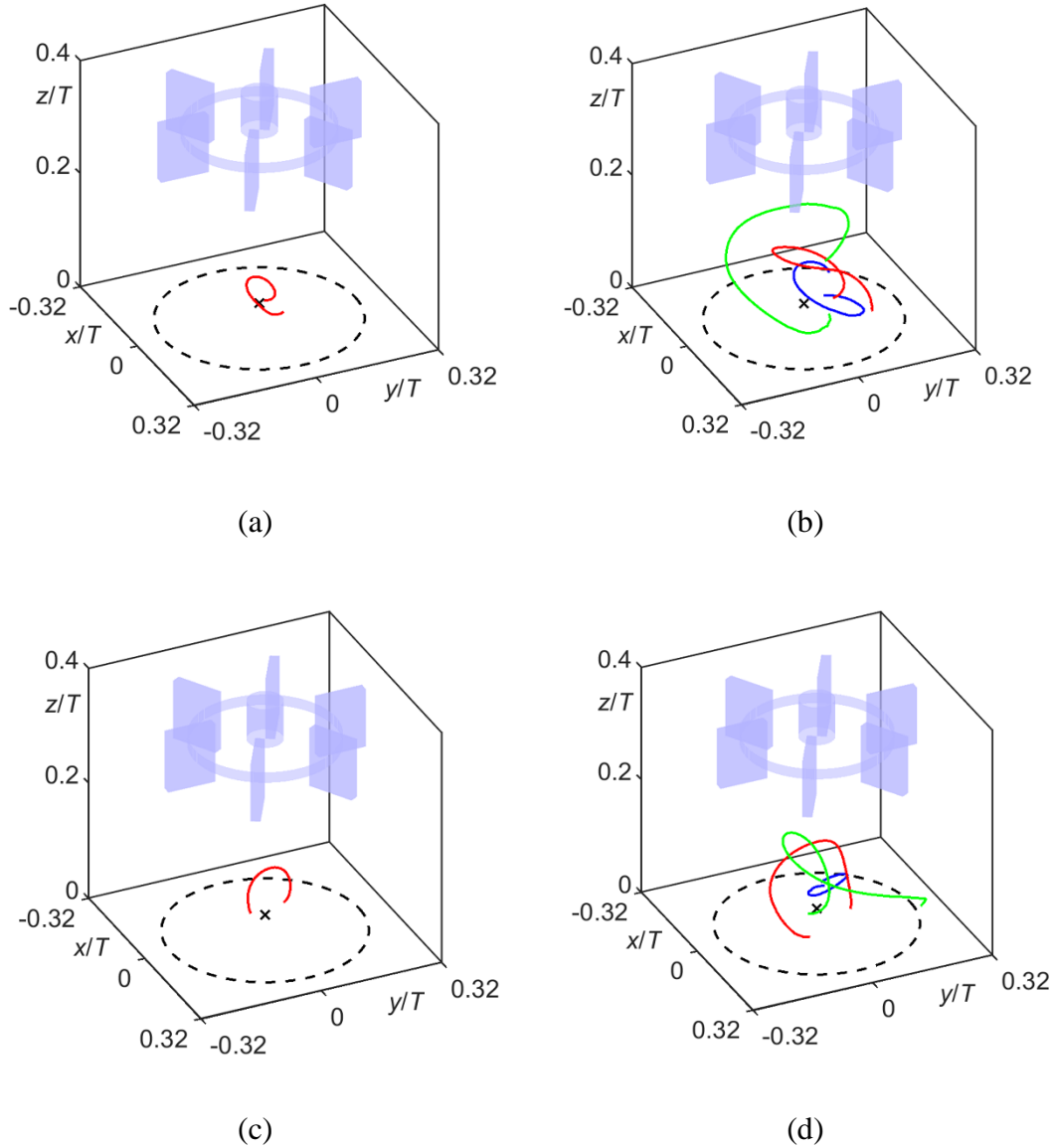
FIGURE 4 Lift-off trajectories of glass and PTFE particles at C=1/3T . (a) Case E15, PTFE, Re = 478 ; (b) case E16, PTFE, Re = 619 ; (c) case E20, glass, Re = 503 ; (d) case E21, glass, Re = 654 . The PTFE and glass particles could be lifted off only once within 60 s at Re = 478 and Re = 503 , as shown in panels (a) and (c). As Reynolds number increases to 619 and 654, the PTFE and glass particles could be lifted off several times within 60 s. Only three lift-off trajectories in different colors are illustrated in panels (b) and (d). The dashed circle on the bottom wall in each panel, with diameter of D , is used for reference. A marker with coordinate (0, 0, 0.5d_p) is shown in each panel.
