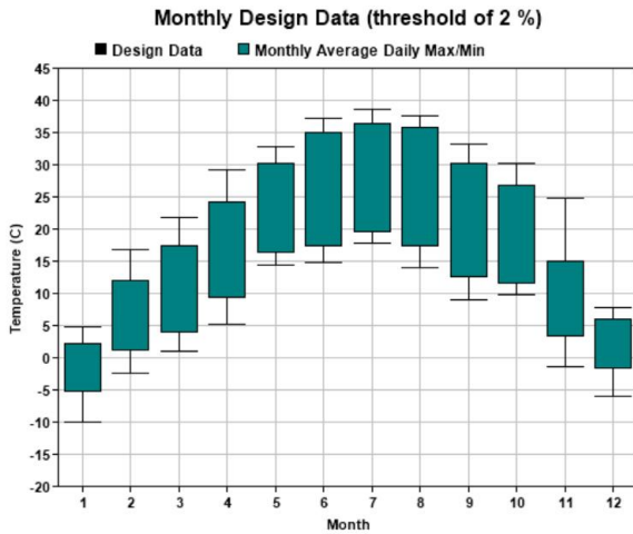
Fig. 3: Average maximum and minimum daily temperatures on a monthly basis
