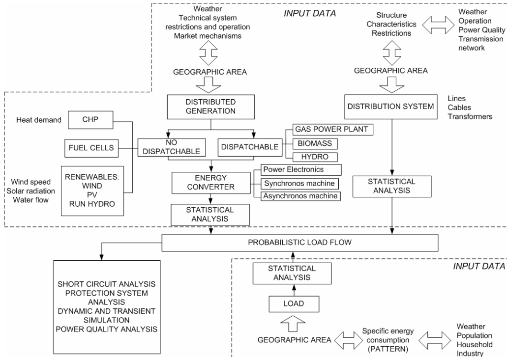
Fig.1. Distribution Power System Analysis Method
