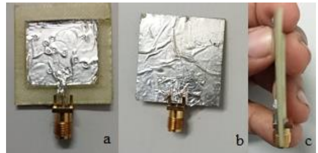
Fig. 5. 3D fabricated antenna: a–patch; b–ground; c–lateral view of antenna
