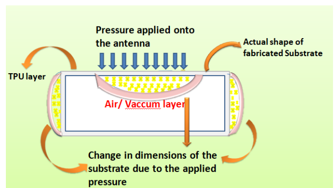
Fig. 2. Representation of the change in the physical dimensions of the antenna with applied pressure
