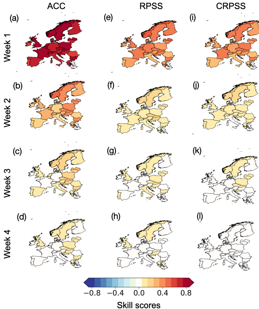
Figure 3. Country-level skill scores for weekly-mean demand-net-wind from the ECMWF model for (a–d) anomaly correlation coefficient, ACC; (e–h) rank probability skill score, RPSS (i–l); and continuous rank probability skill score, CRPSS. Definitions of skill scores are given in Sect. 2.
