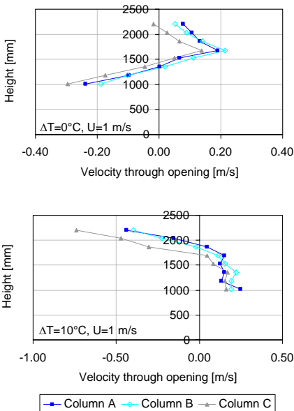
Figure 5.30. Change in velocity profiles with increase in temperature. Angle = 0°. Positive values indicate an ingoing flow.
