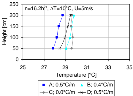
Figure 5.3. Temperature gradients measured in cross-ventilation with U=5\text{m/s} . Incidence angle = 0^\circ .
