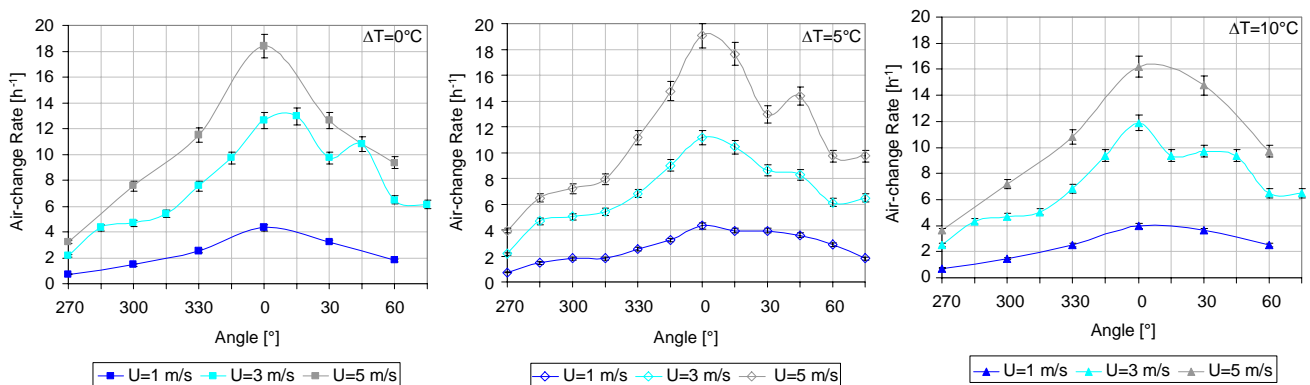
Figure 5.7. Effect on the air-change rate from changing the wind velocity at different incidence angles and temperature differences.
