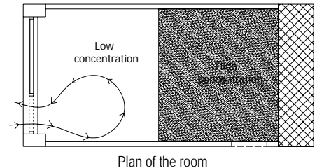
Figure 4.26. Problem with incomplete mixing in the room because of a horizontal gradient.
