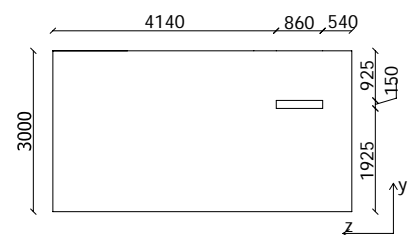
Figure 4.7. Positions and sizes of the openings in cross-ventilation. Dimensions in mm.
