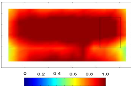
Figure 4.9. C_p -values measured at the front wall on the closed building with an incidence angle of 0^\circ . The position of the window during the experiments with single-sided ventilation is marked on the building.
