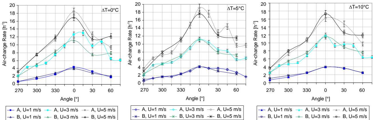
Figure 5.13. Differences in air-change rates between set-up A and set-up B as a function of different velocities at fixed temperature differences.
