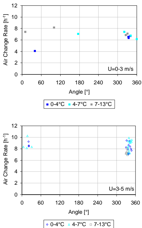
Figure 5.58. Air change rate as a function of temperature difference at velocities from 0-3 m/s and 3-5 m/s.
