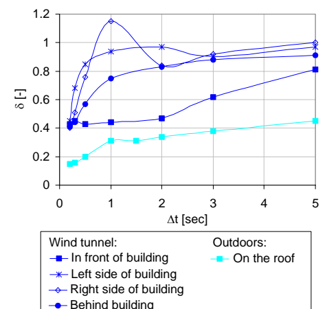
Figure 3.38. \delta -values from the lagged scatterplots made outside the buildings. In the wind tunnel h=3m is used.
