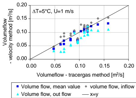
Figure 5.23. Coherence between volume flows found from the decay method and from calculations of measured velocities in the opening.
