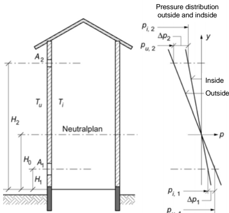
Figure 1.9. Pressure difference around the neutral plane in a building ventilated only by thermal buoyancy. /By og Byg 202/
