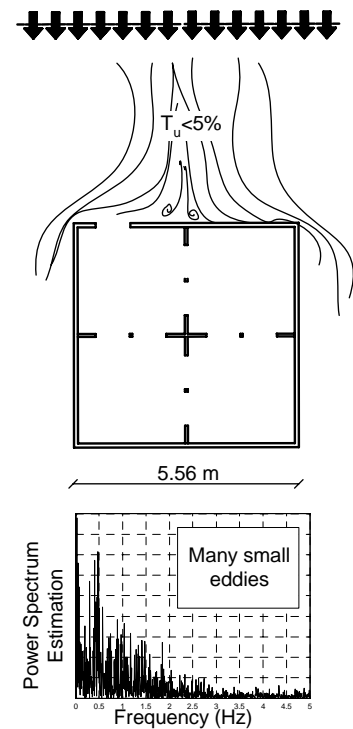
Figure 5.64. Characteristics found for mechanical wind – building length = 5.56m..
