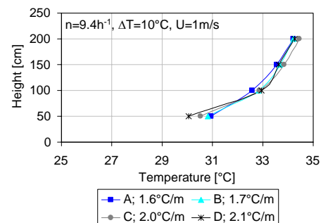
Figure 5.21. Temperature gradients measured in single-sided ventilation with U=1\text{m/s} . Incidence angle = 0^{\circ} .
