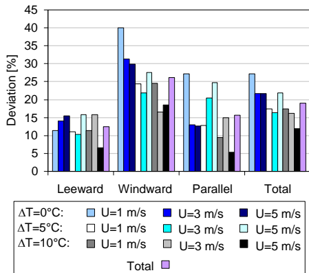
Figure 5.47. Errors found for each case divided into leeward, windward or parallel.
