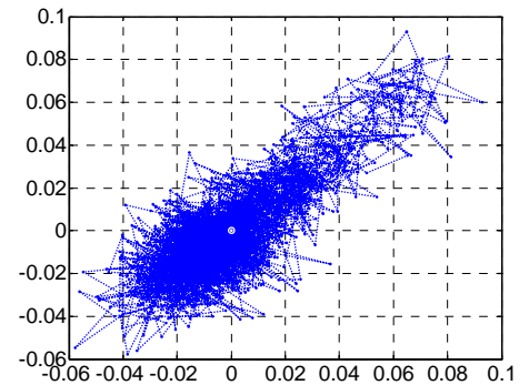
Figure 3.36. Lagged scatterplot for \Delta t=0.2 second in point 15, h=3m , in wind tunnel.
