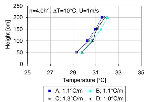
Figure 5.2. Temperature gradients measured in cross-ventilation with U=1\text{m/s} . Incidence angle = 0^\circ .
