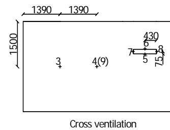
Figure 5.15. Positions of pressure measurement at the front wall (wall facing the wind when \beta=0^\circ ). Number (9) shows the point at the opposite side. Points around the openings are app. 50 mm away from the edge of the opening. Dimensions in mm.
