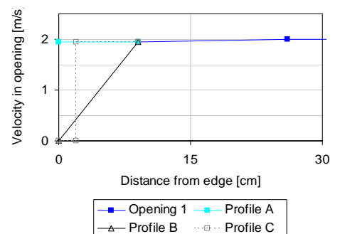
Figure 4.33. Three suggestions for velocity profiles in the area between the vertical edge and the measurement 9 cm away.
