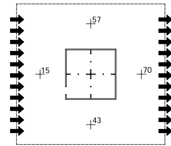
Figure 3.20. Measurement points for "free wind" in the wind tunnel. All points are 2.78 m away from the building.
