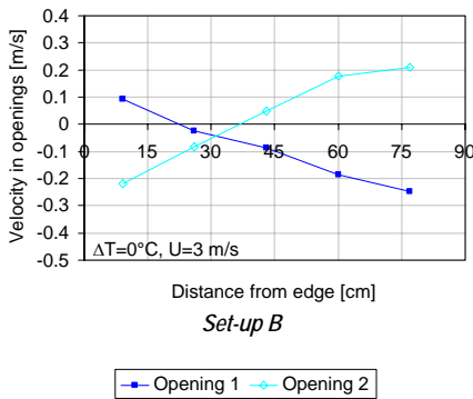
Figure 5.9. Velocity profiles from cross set-ups A and B at \beta=270^\circ with a temperature difference of 0^\circ\text{C} and a velocity of 3 m/s.
