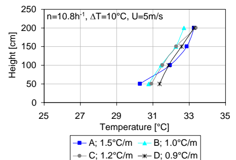
Figure 5.22. Temperature gradients measured in single-sided ventilation with U=5\text{m/s} . Incidence angle = 0^{\circ} .
