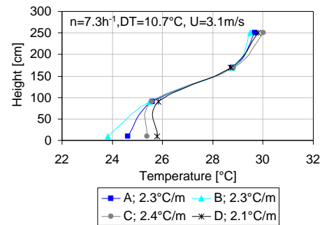
Figure 5.55. Temperature gradients measured in case 73. Incidence angle = 331°.
